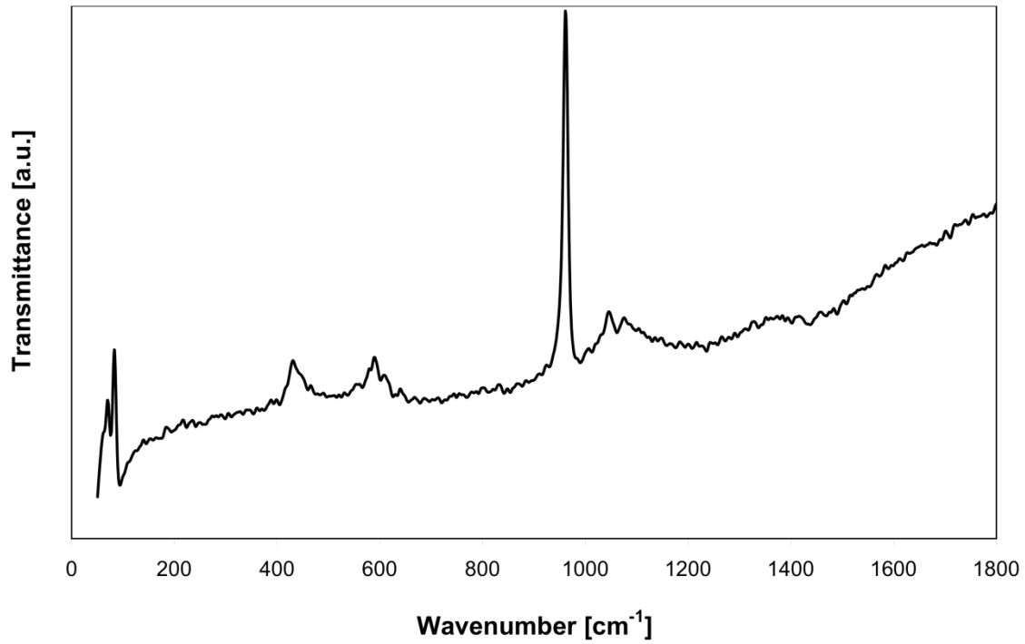
Figure S4: Raman-spectrum of HAp.
