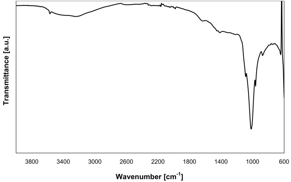
Figure S3: FT-IR spectrum of HAp.
