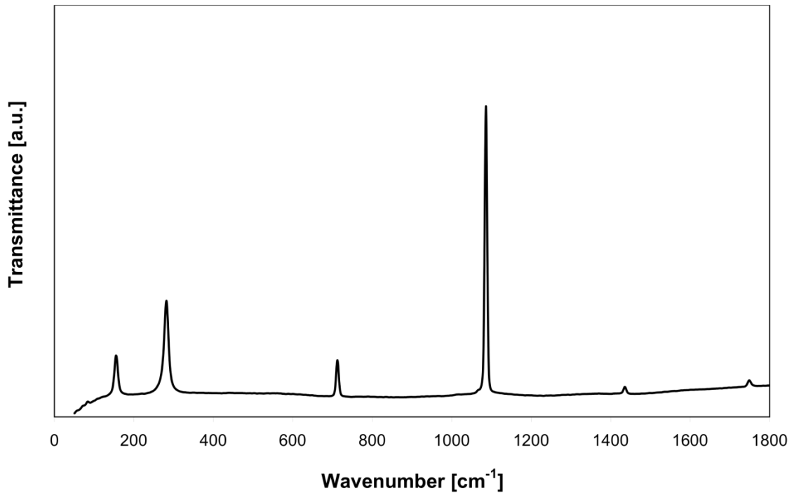
Figure S2: Raman spectrum of CaCO 3 .
