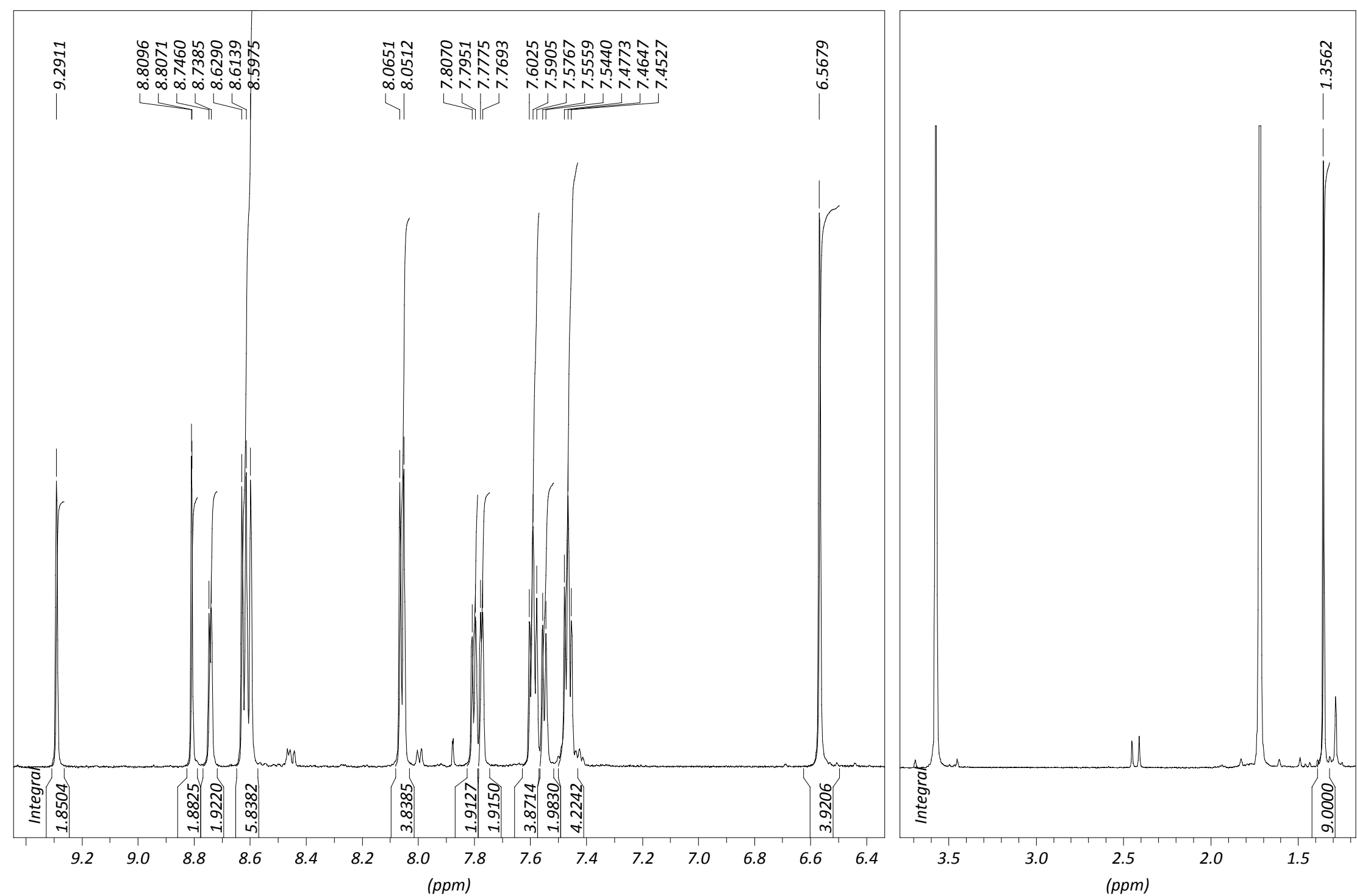
1H-NMR-spectrum of 5a
