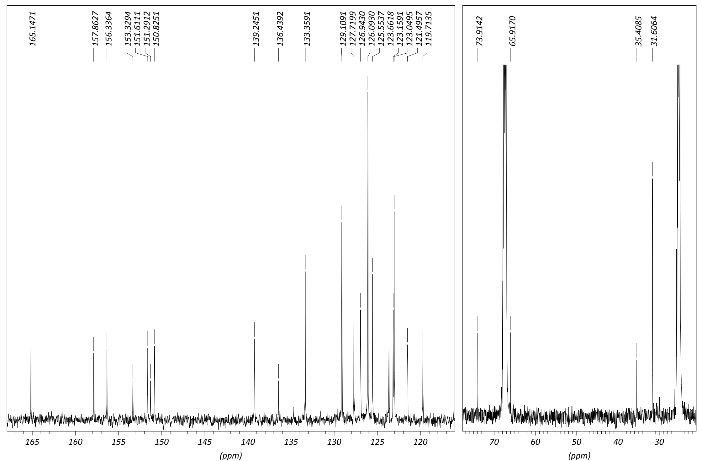
^{13}\text{C} -NMR-spectrum of 5b
