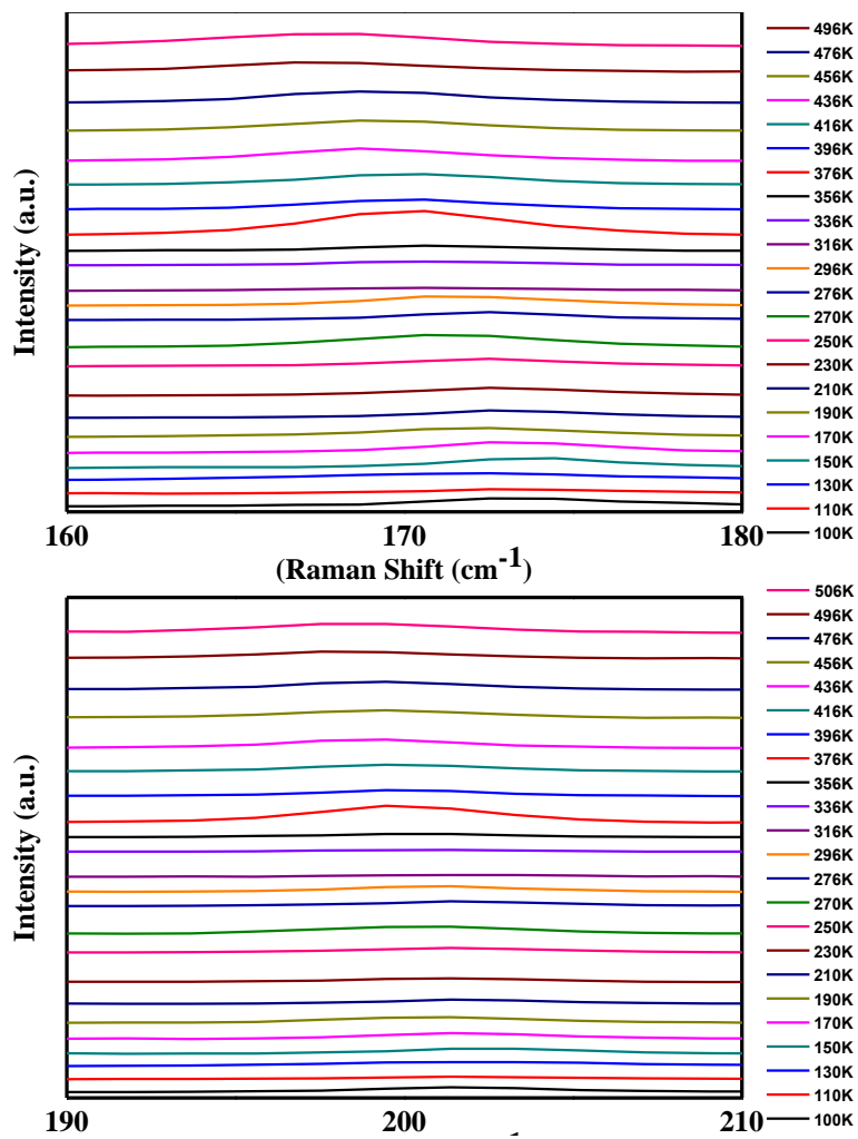
Figure S3: The normalized Raman spectra of PtSe 2 nanosheets at different temperatures for two modes.
