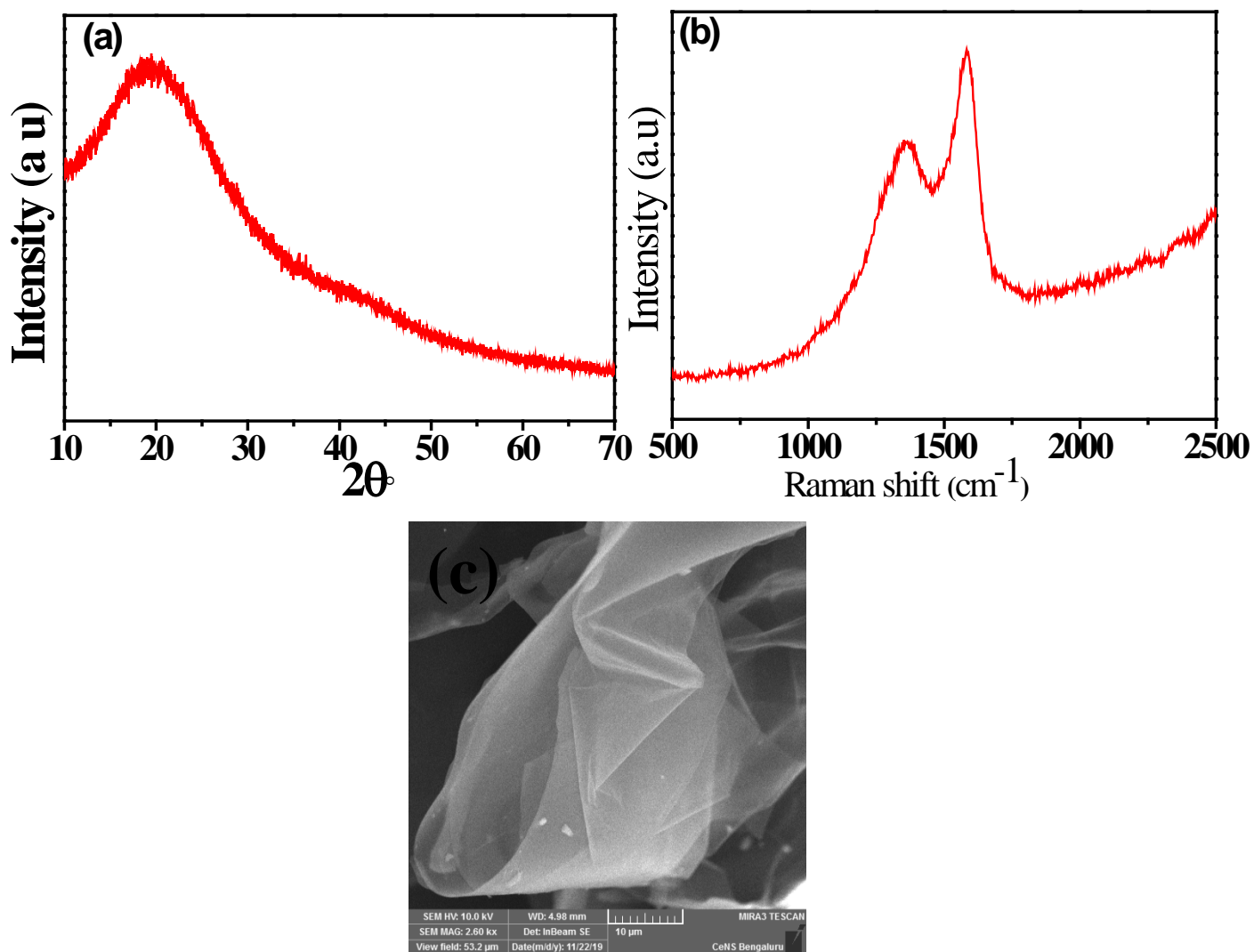
Figure S1: (a) XRD pattern, (b) Raman spectrum, and (c) SEM image of rGO nanosheets synthesized at 400 °C.
