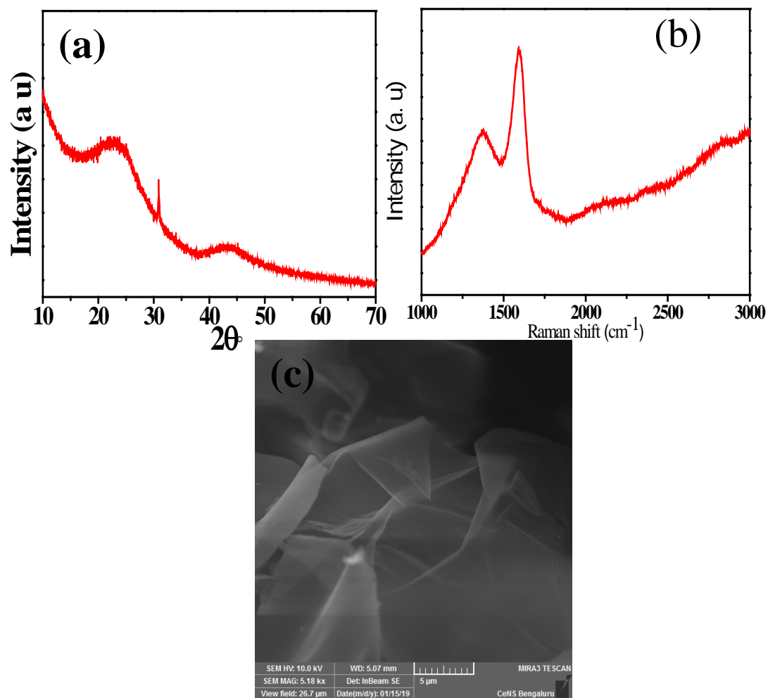
Figure S2: (a) XRD pattern, (b) Raman spectrum, and (c) SEM image of rGO nanosheets synthesized at 600 °C.
