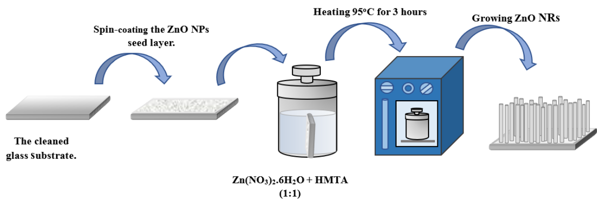
Figure S1: Synthesis of ZnO NRs.
