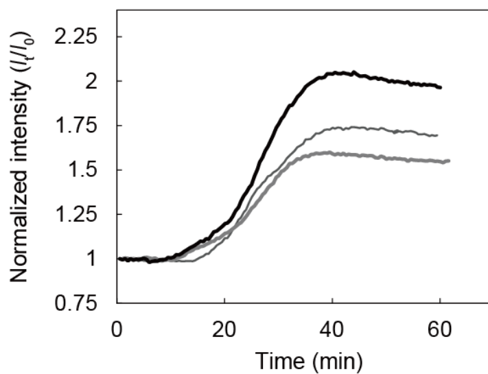
Figure S1: Change in reflected light intensity during the electroless nickel plating reaction. The reflected light intensity was measured at 55 nm. The profiles obtained using three different optical fibers are shown.
