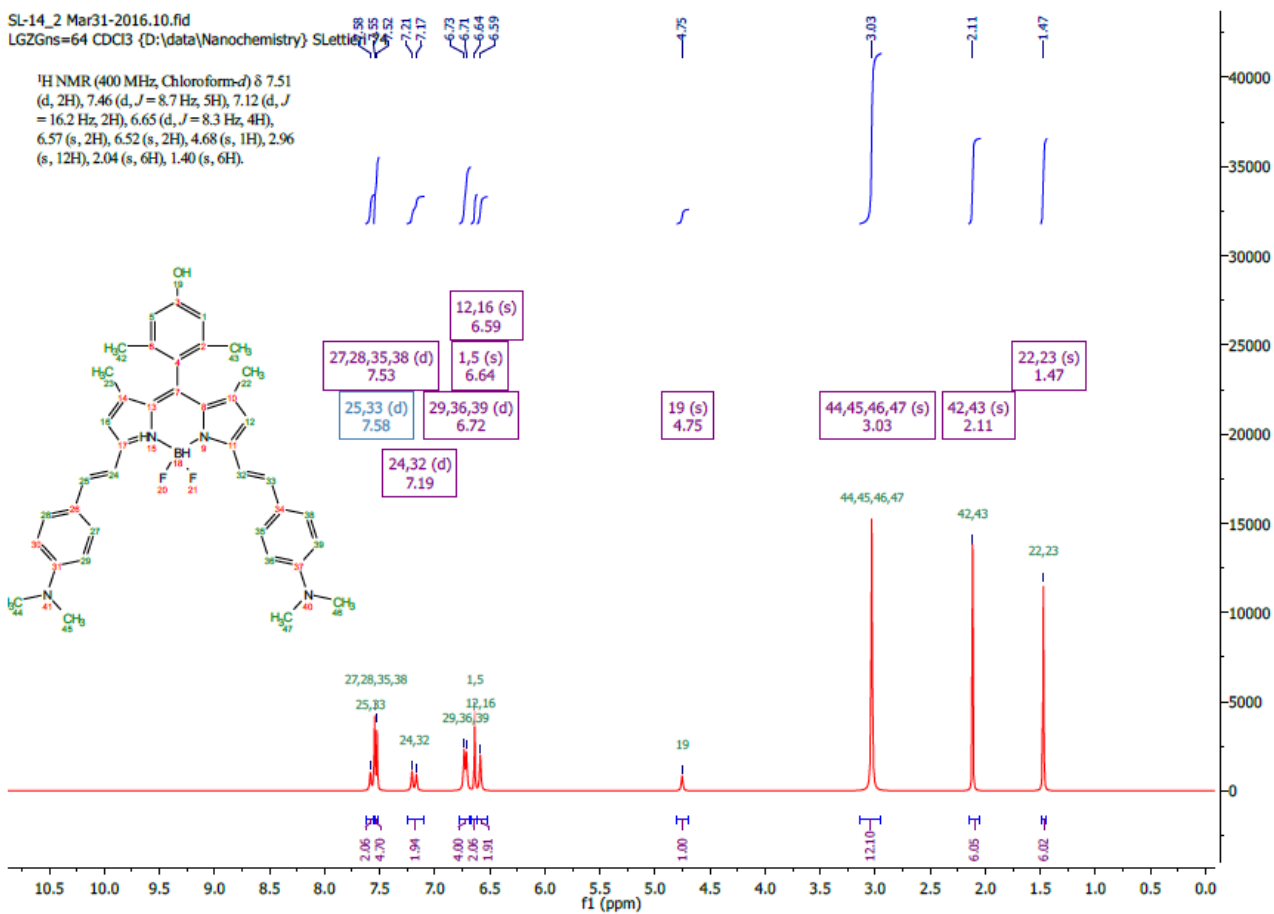
Figure S3: 1 H NMR spectrum in Chloroform- d of BODIPY 3.
