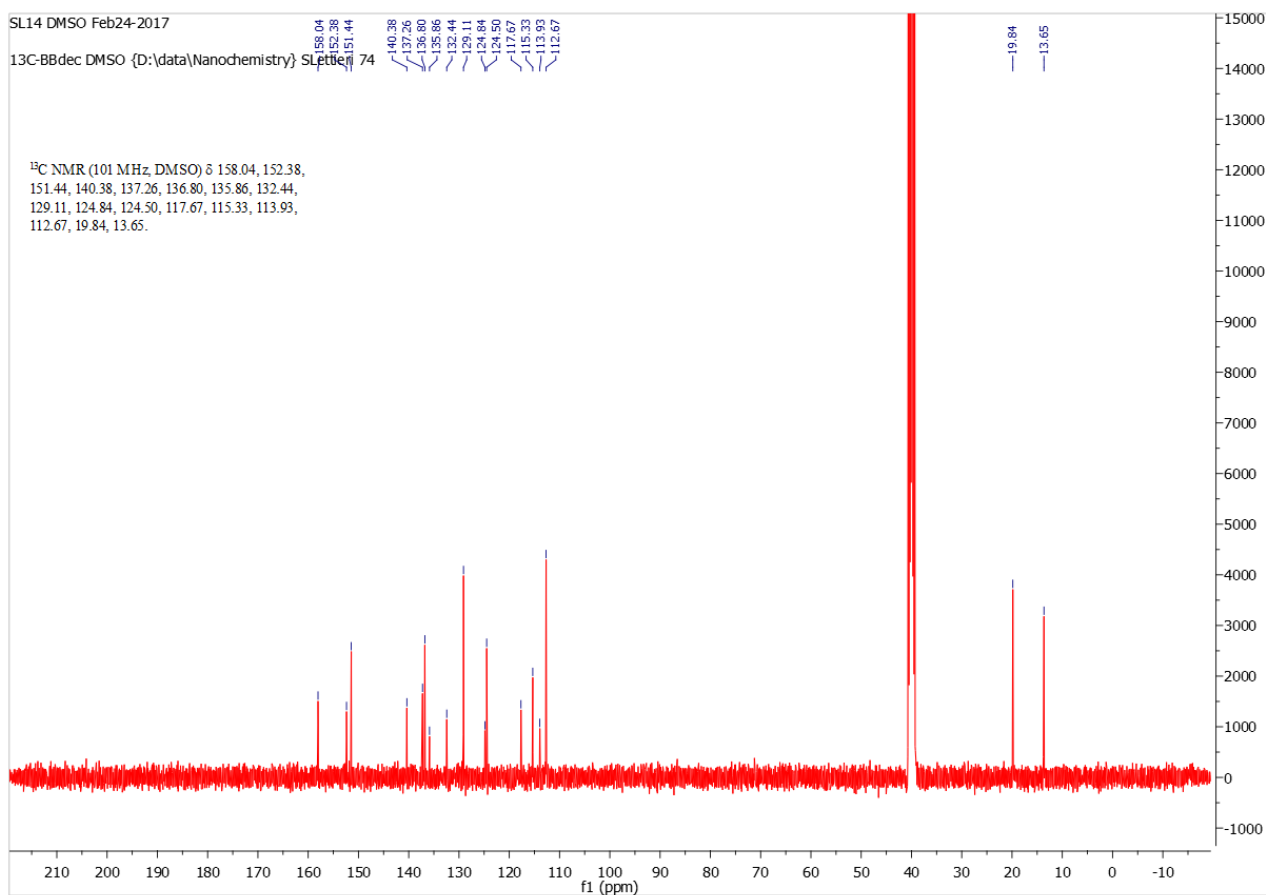
Figure S4: ^{13}\text{C} NMR spectrum in DMSO- d_6 of BODIPY 3 .
