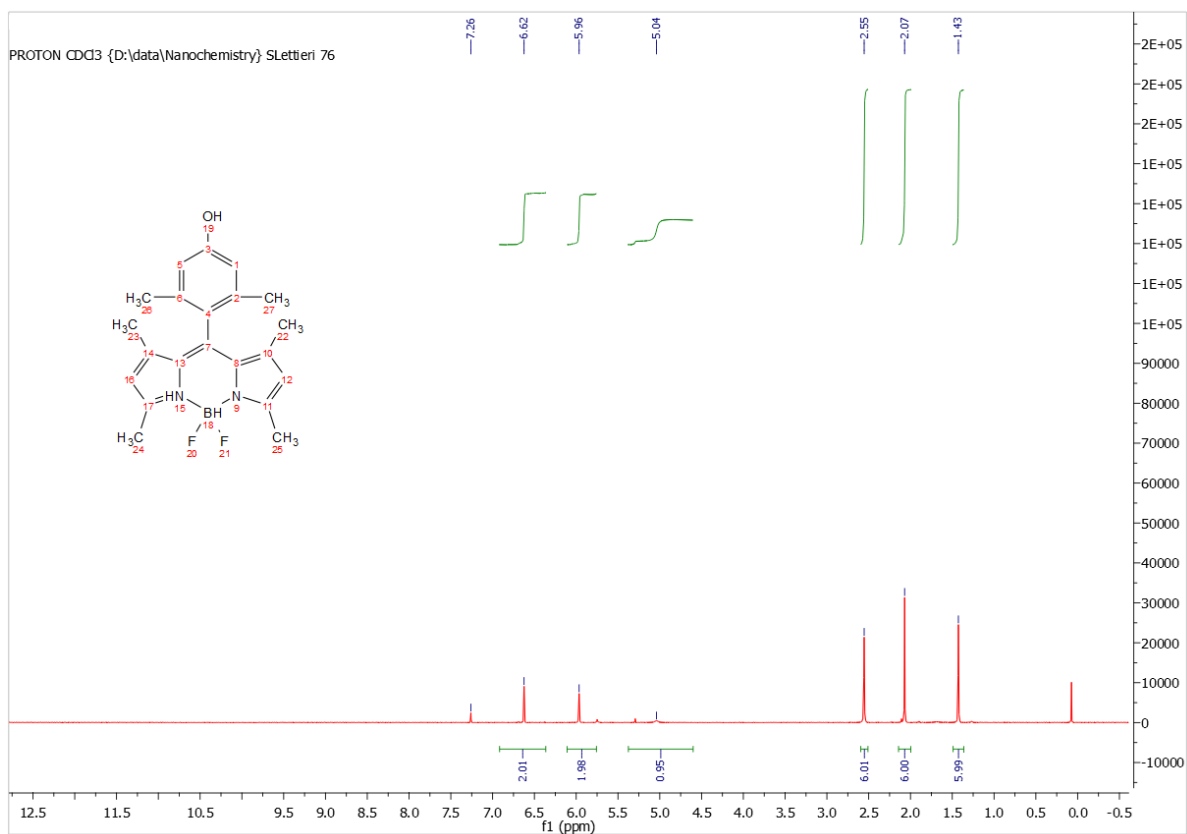
Figure S2: 1 H NMR spectrum in Chloroform- d of compound 2 .
