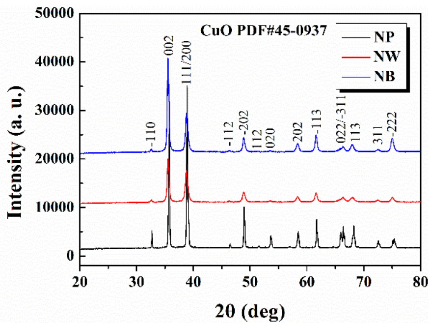
Figure S1: X-ray diffraction profile for CuO nanoparticles (NP), nanowires (NW) and nanobelts (NB).
