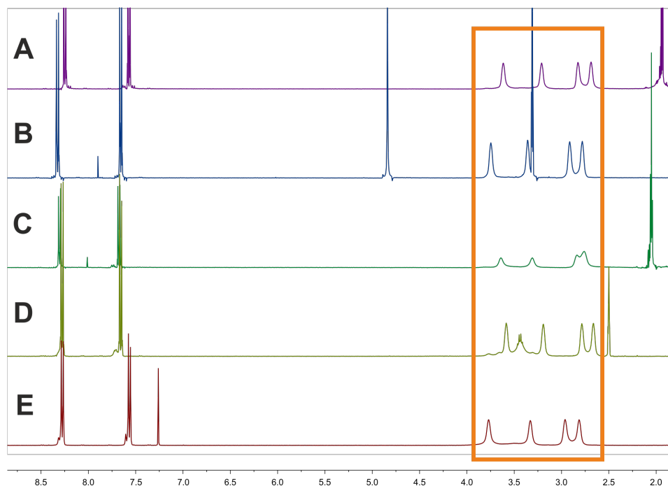
Figure 1: ^1\text{H} NMR spectra of compound 3a measured in five different solvents: (A) acetonitrile- d_3 , (B) methanol- d_4 , (C) acetone- d_6 , (D) DMSO- d_6 and (E) \text{CDCl}_3 (orange: region of interest).
