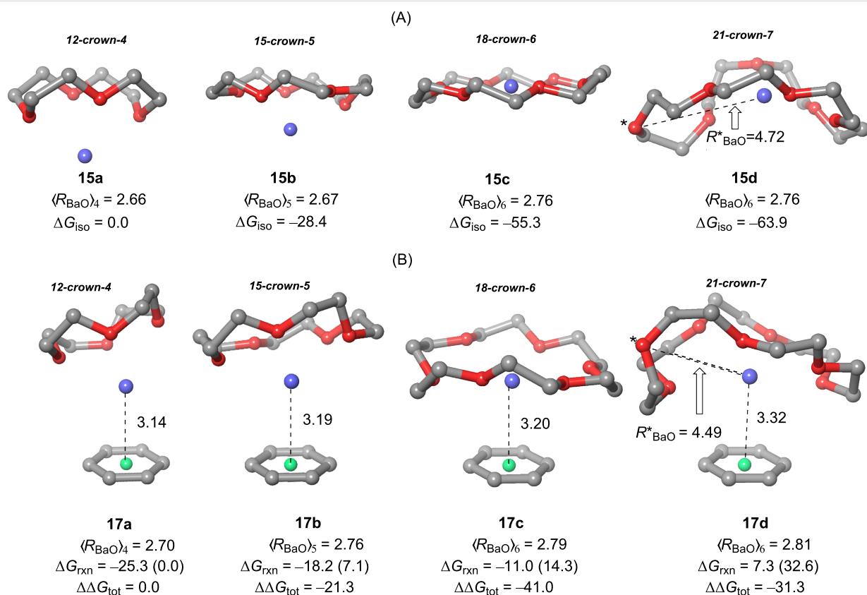
Figure 4: Fully optimized geometries (B3LYP-D3BJ/6ccrow-311++G**+DefTZVPP(Ba) level of theory) of \text{Ba}^{2+} -crown ethers 15a–d (A) and phenyl- \text{Ba}^{2+} -crown ether complexes 17a–d (B). Barium cations are represented in dark blue. Descriptors \langle R_{\text{BaO}} \rangle_n denote the average Ba–O bond distances (in Å) for the different crown ethers. Distances between \text{Ba}^{2+} and the ring points of electron density of benzene (in green) are also gathered in (B). \Delta G_{\text{iso}} and \Delta G_{\text{rxn}} terms stand for the Gibbs energies (in kcal/mol) described in Scheme 2 and have been calculated according to Equation 3 and Equation 4. Numbers in parentheses are the relative \Delta G_{\text{rxn}} energies with respect to complex 17a . \Delta \Delta G_{\text{tot}} energies have been calculated according to Equation 5. Hydrogen atoms have been omitted for clarity.
