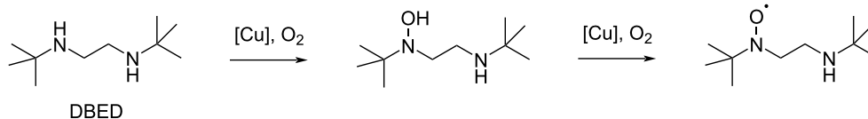
Scheme 19: In situ generation of N -oxyl radicals from DBED.
