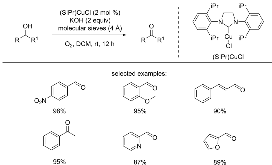
Scheme 20: (SIPr)CuCl-catalyzed aerobic oxidation of alcohols.
