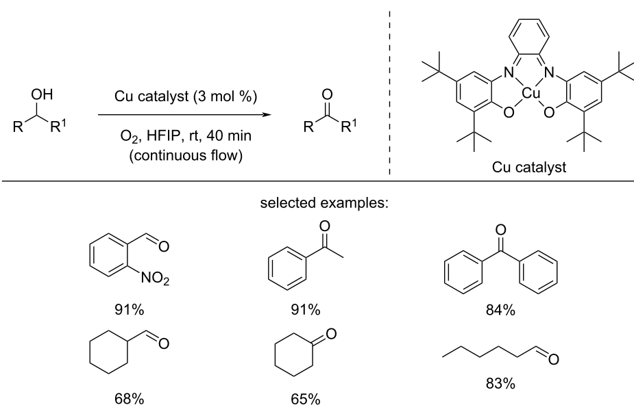
Scheme 21: Base- and nitroxyl radical-free Cu-catalyzed aerobic oxidation of alcohols under continuous-flow conditions.
