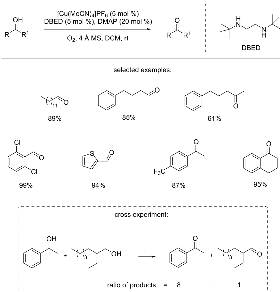
Scheme 18: TEMPO-free Cu-catalyzed aerobic oxidation of alcohols reported by Arndtsen and Lumb [81].
