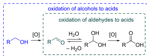
Scheme 22: Carboxylic acids as products of aldehyde and alcohol oxidations – general mechanism.
