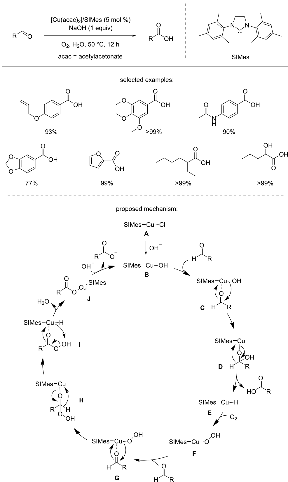
Scheme 23: The first homogeneous Cu-catalyzed aerobic oxidation of aldehydes.
