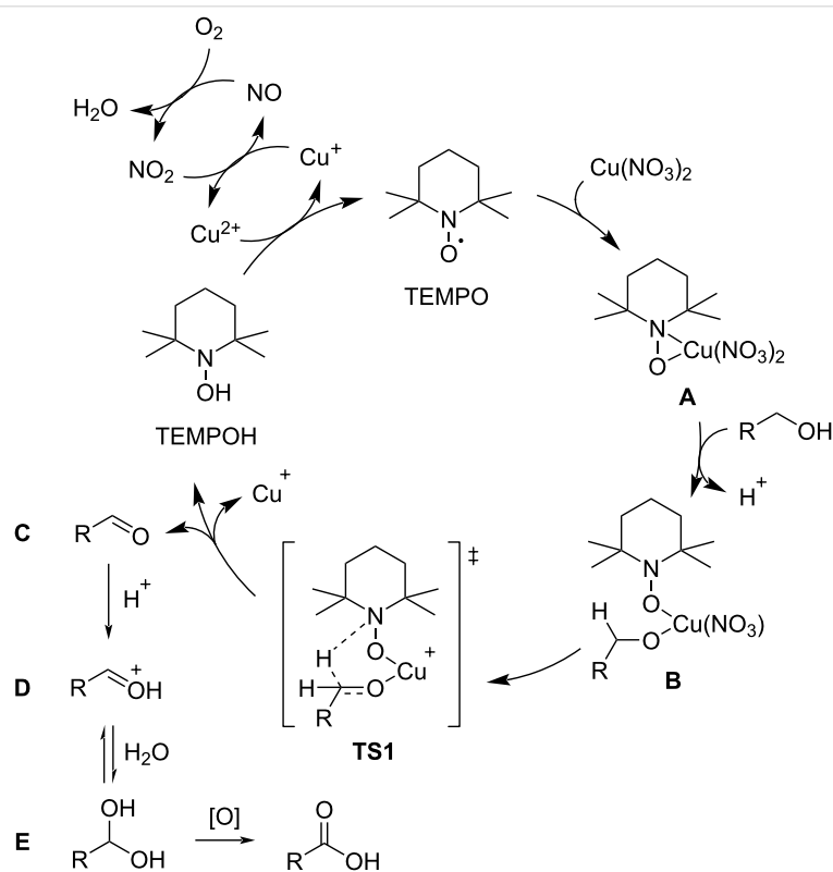
Scheme 27: Proposed mechanism for the \text{Cu(NO}_3)_2 \cdot 3\text{H}_2\text{O} /TEMPO/ \text{KHSO}_4 -catalyzed direct conversion of alcohols to acids.
