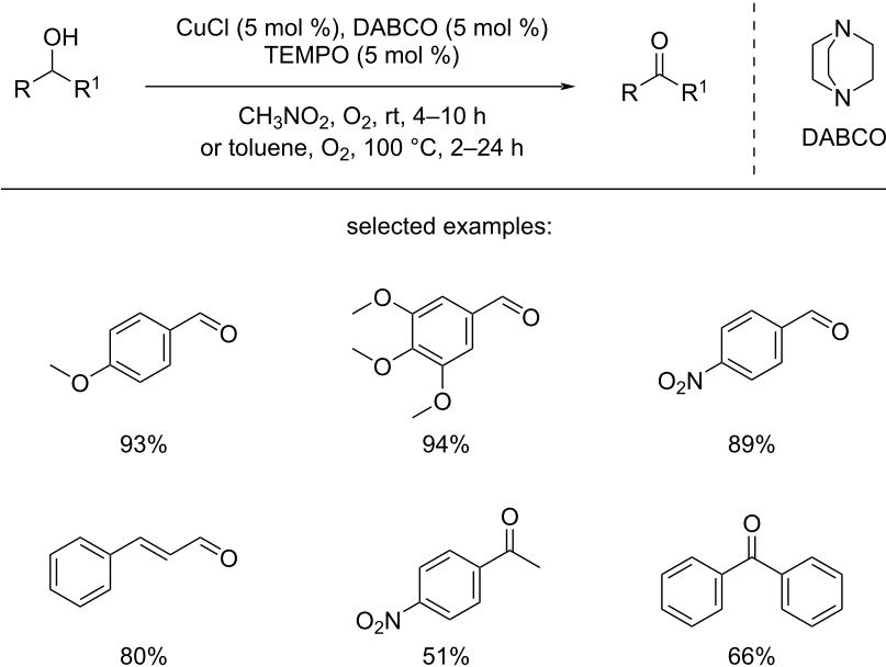
Scheme 6: The CuCl/DABCO/TEMPO system for the aerobic oxidation of activated alcohols.
