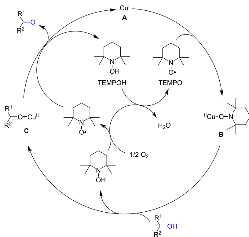
Scheme 4: Revisited mechanism of the Cu/TEMPO-catalyzed aerobic oxidation of alcohols by Sheldon et al. [59].
