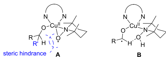
Figure 1: Possible explanation for the lack of reactivity of secondary alcohols proposed by Sheldon et al. [61].
