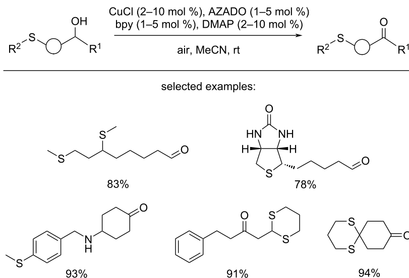
Scheme 10: The Cu/AZADO catalytic system for the aerobic oxidation of sulfur-containing alcohols.
