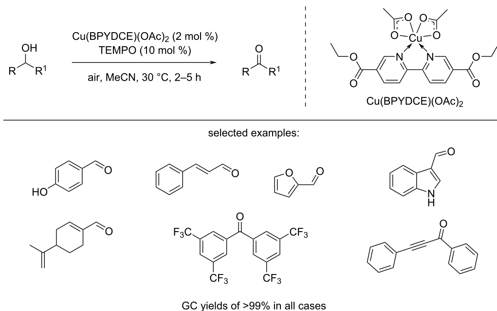
Scheme 11: Cu(BPYDCDE)(OAc) 2 /TEMPO-catalyzed external base-free aerobic oxidation of alcohols.
