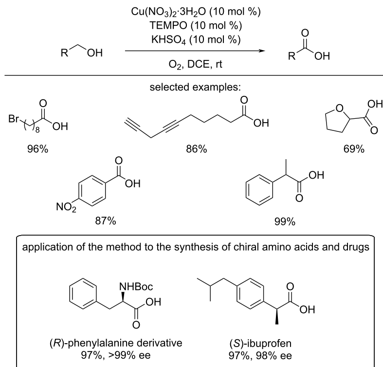
Scheme 26: \text{Cu(NO}_3)_2 \cdot 3\text{H}_2\text{O} /TEMPO/ \text{KHSO}_4 -catalyzed direct oxidation of alcohols to carboxylic acids.
