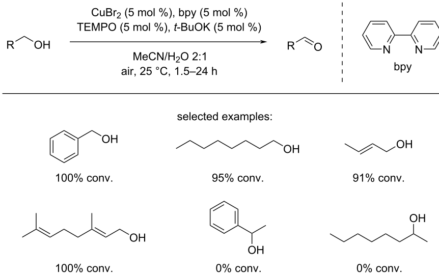
Scheme 5: CuBr 2 /bpy/TEMPO-catalyzed oxidation of primary alcohols to aldehydes under air.
