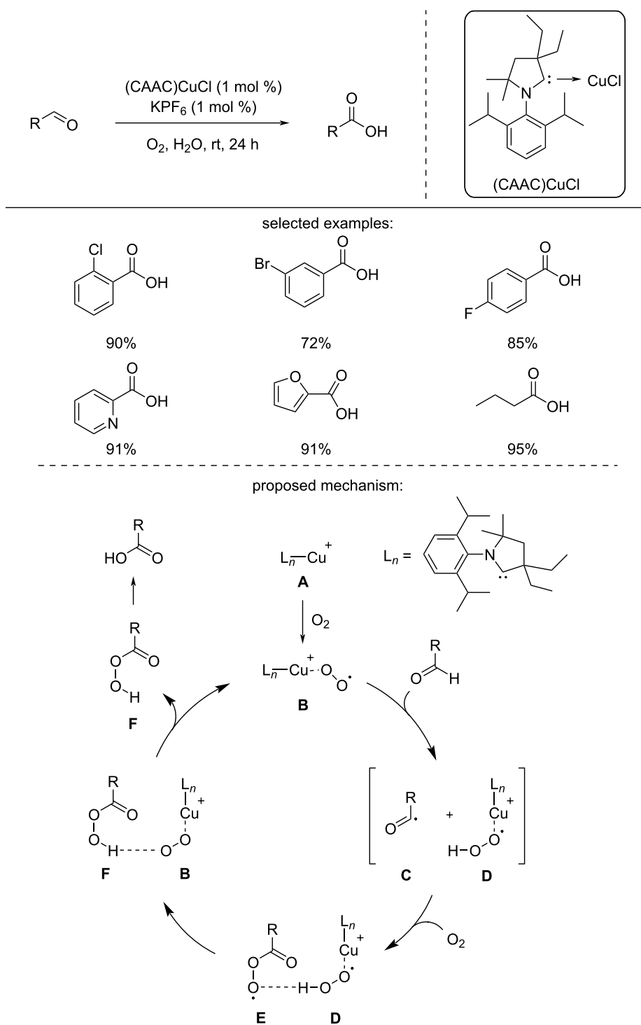
Scheme 24: (CAAC)CuCl-catalyzed aerobic oxidation of aldehydes.
