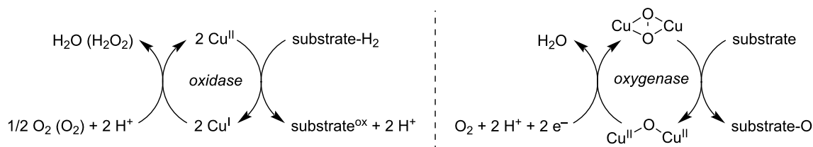
Scheme 1: Oxidase- and oxygenase-like copper-based oxidation reactions.
