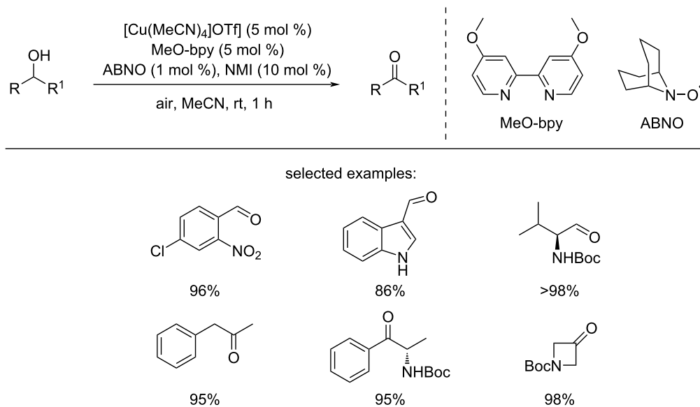
Scheme 8: The Cu/ABNO catalytic system for the aerobic oxidation of both primary and secondary alcohols.
