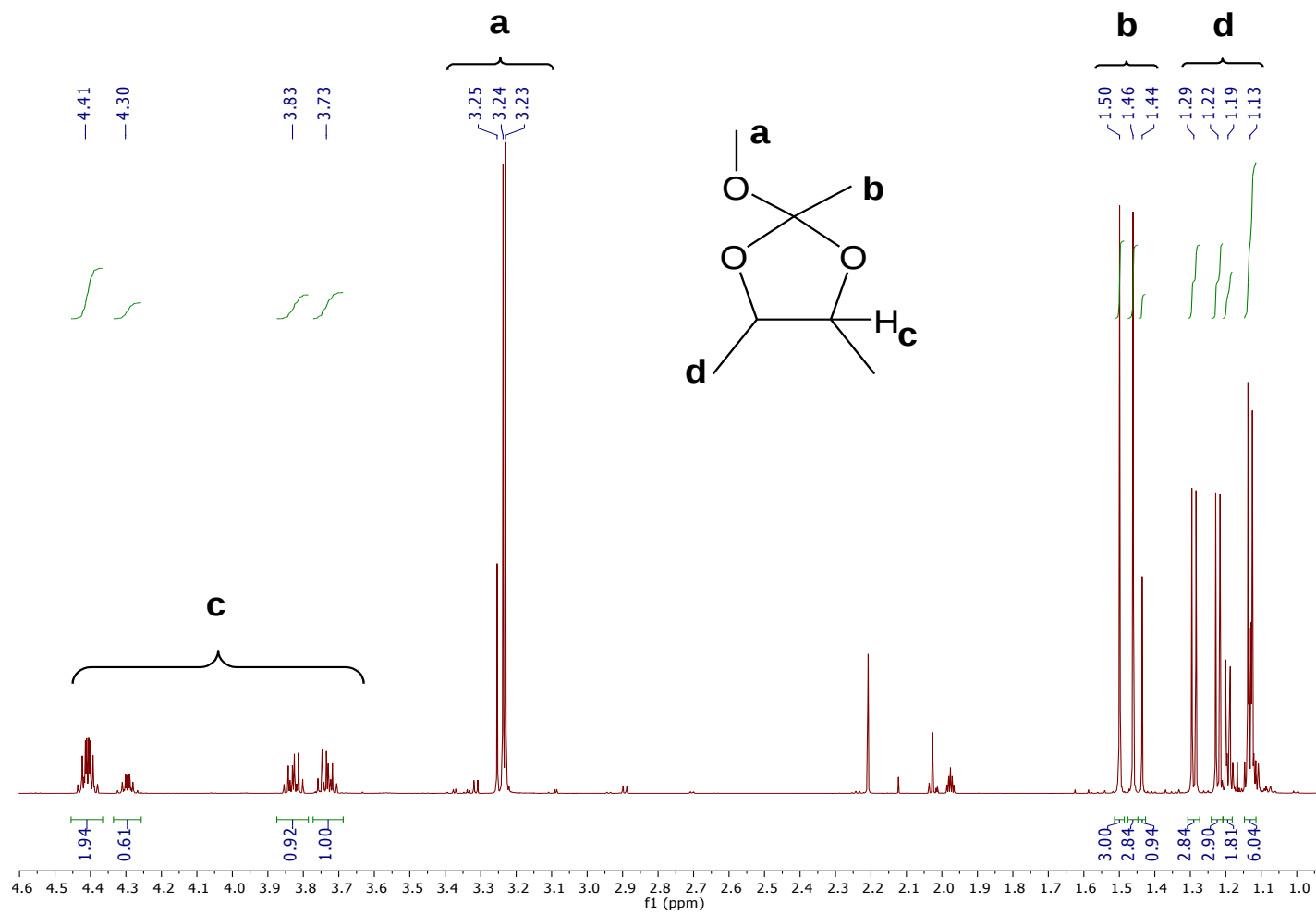
500 MHz ^1\text{H} NMR spectrum of a mixture of 10 , 11 and 14 in \text{CD}_3\text{CN} .
