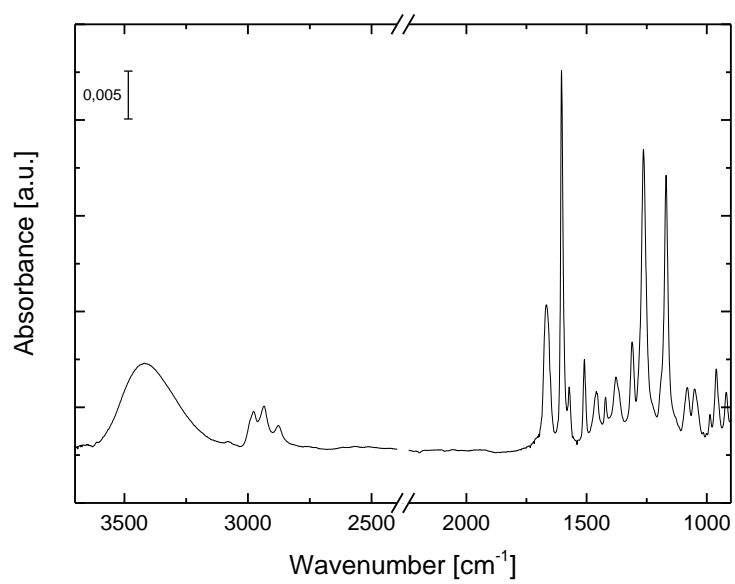
Figure S3: IRRA spectrum of 2-hydroxy-4'-(2-hydroxyethoxy)-2-methylpropiophenone.
