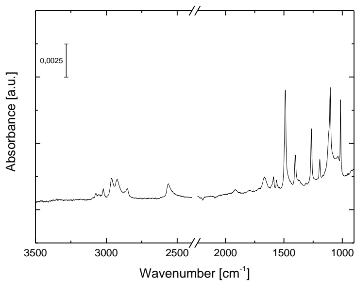
Figure S2: IRRA spectrum of Tetrakis(4-thiolphenyl)-methane (TPM-SH).
