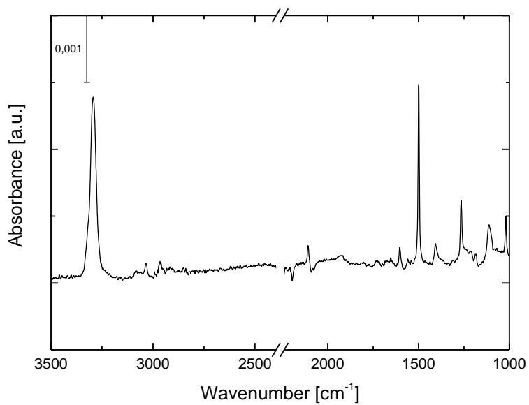
Figure S1: IRRA spectrum of Tetrakis(4-ethynyl-phenyl)methane (TPM-alkyne).
