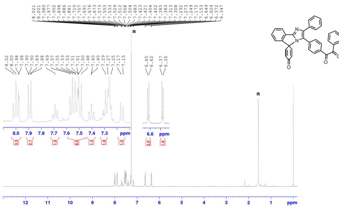
Figure S3. ^1\text{H} NMR spectrum of the isomer B of Benzil-PIC in \text{CDCl}_3 (* solvent peaks).
