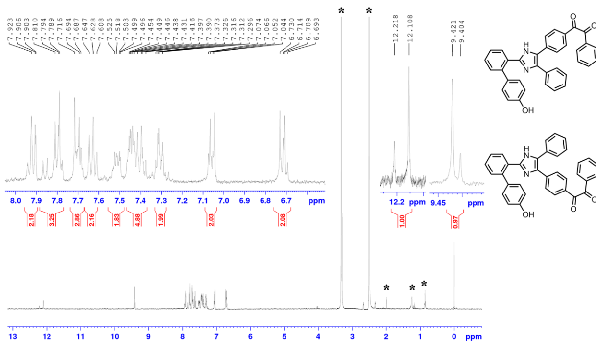
Figure S1. ^1\text{H} NMR spectrum of 2 in \text{DMSO}-d_6 (* solvent peaks).
