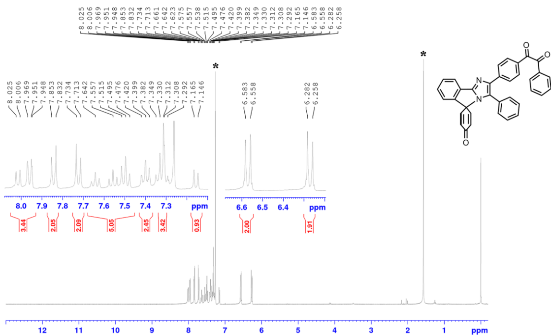
Figure S2. ^1\text{H} NMR spectrum of the isomer A of Benzil-PIC in \text{CDCl}_3 (* solvent peaks).
