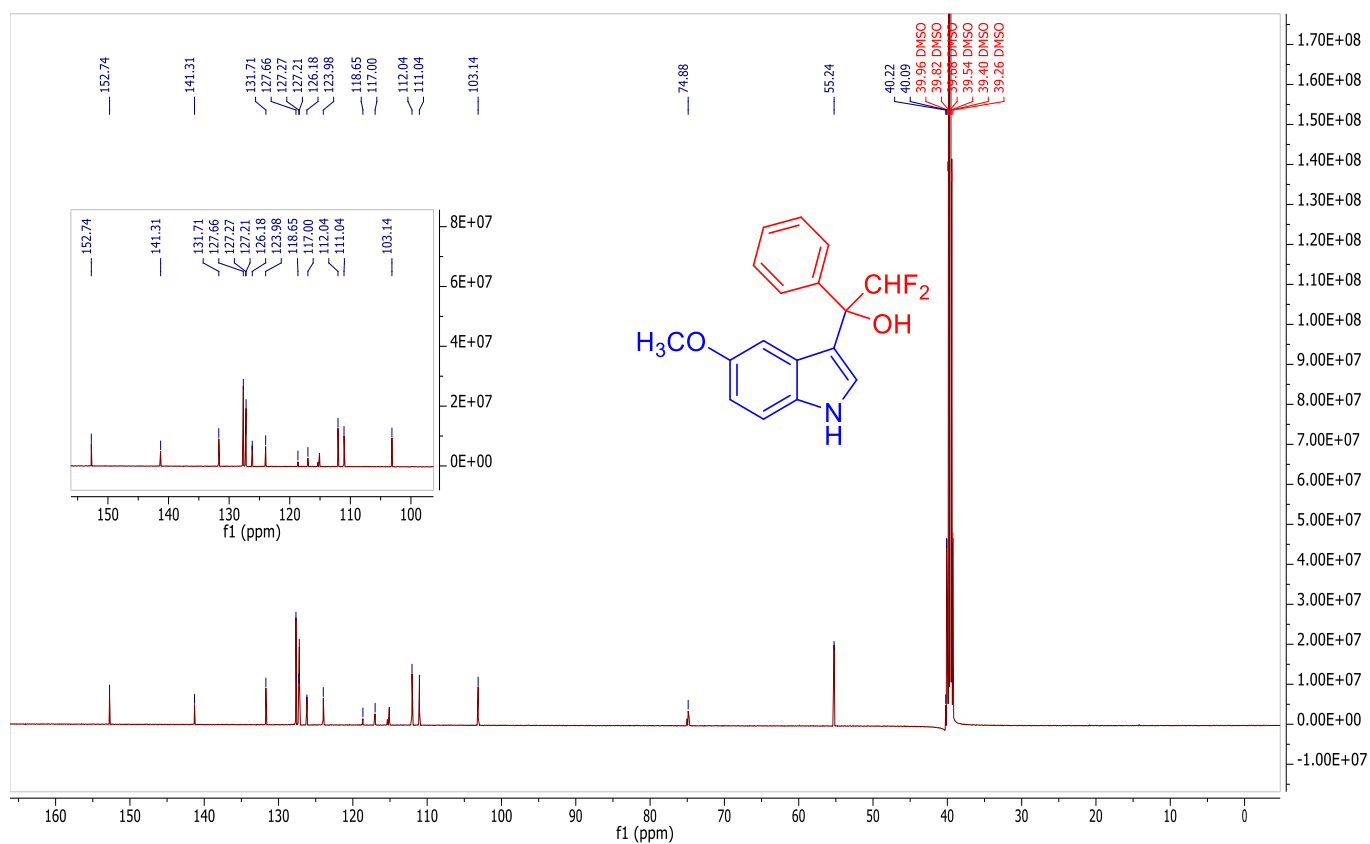
Figure S10. ^1\text{H} (600 MHz) and ^{13}\text{C} (151 MHz) Spectra of 2,2-tifluoro-1-(5-methoxy-1 H -indol-3-yl)-1-phenylethan-1-ol ( 3i )
