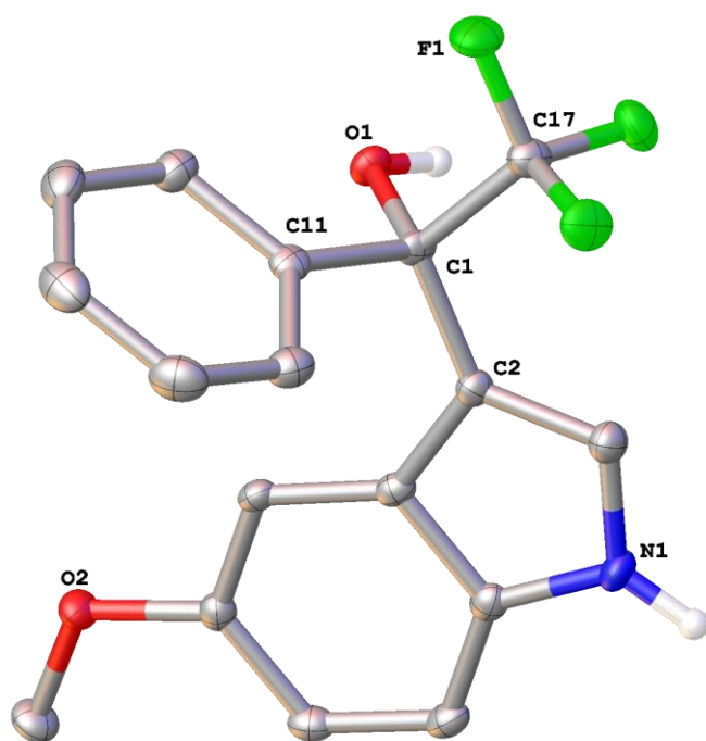
Figure S1. ORTEP-type plot of the molecular structure of 3a (asymmetric unit) in the single crystal lattice at 100(2) K. The thermal ellipsoids are set at 50% probability.
