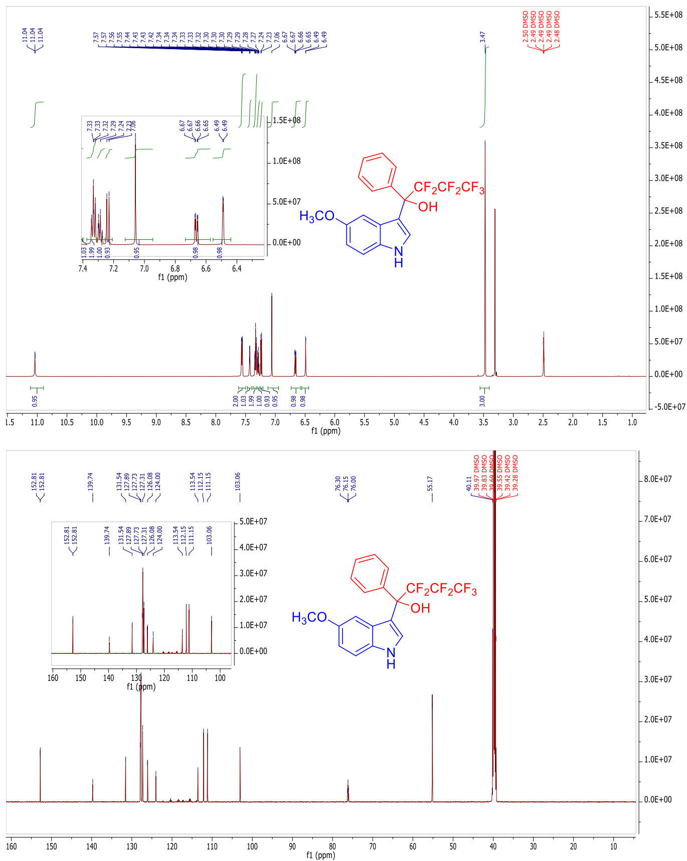
Figure S13. 1 H (600 MHz) and 13 C (151 MHz) Spectra of 2,2,3,3,4,4,4-heptafluoro-1-(5-methoxy-1 H -indol-3-yl)-1-phenylbutan-1-ol ( 3o )
