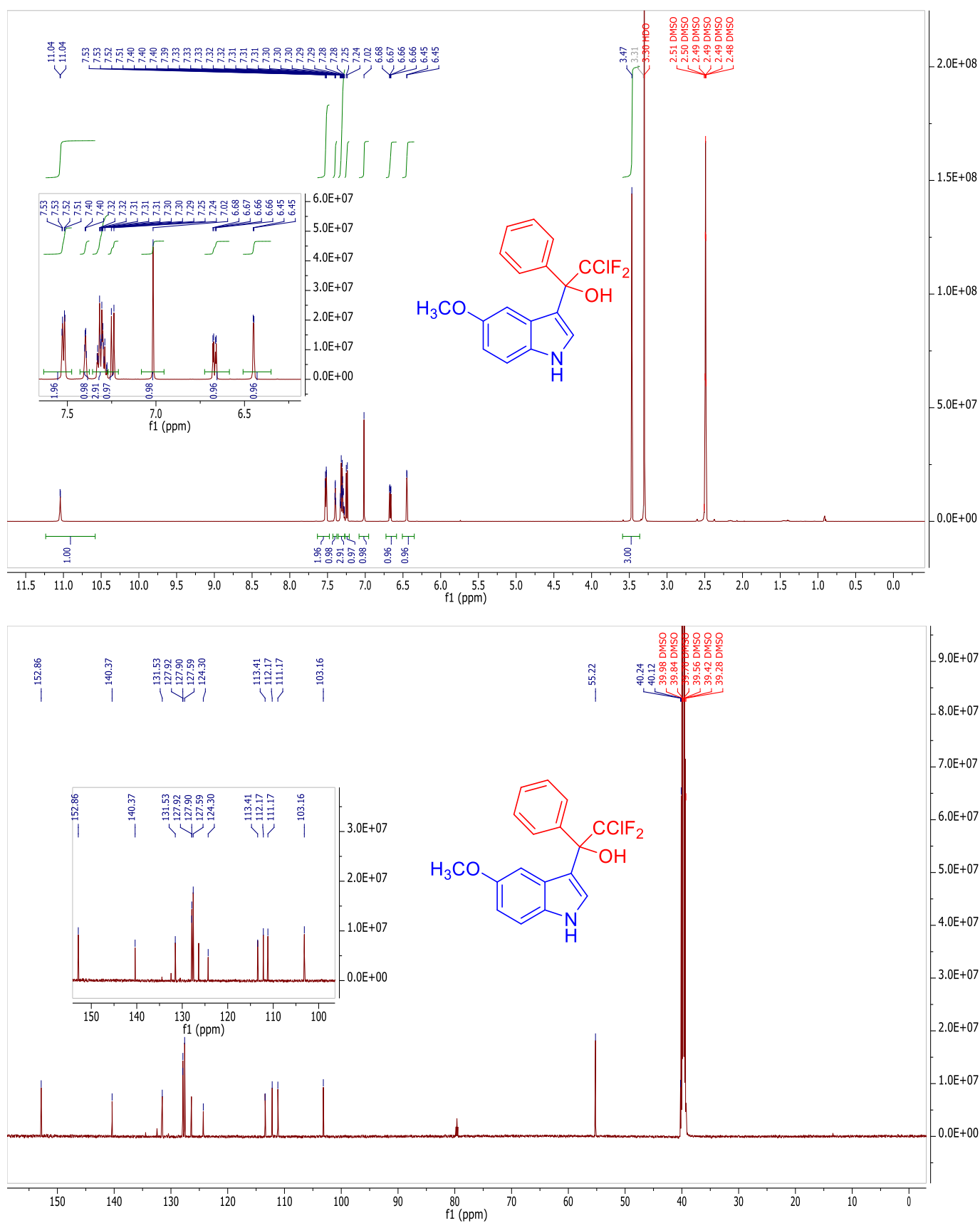
Figure S11. 1 H (600 MHz) and 13 C (151 MHz) Spectra of 2-chloro-2,2-difluoro-1-(5-methoxy-1 H -indol-3-yl)-1-phenylethan-1-ol ( 3m )
