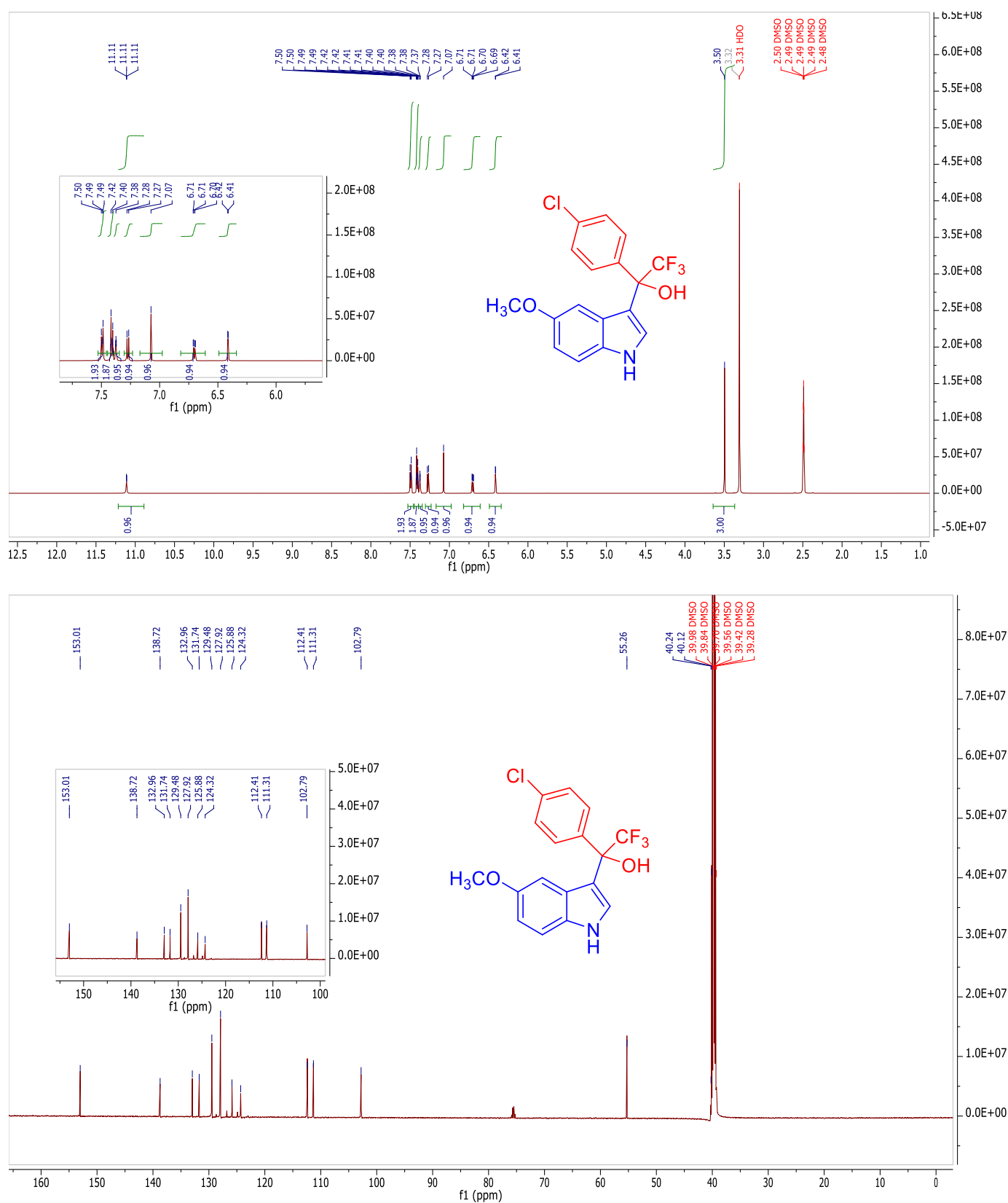
Figure S4. 1 H (600 MHz) and 13 C (151 MHz) Spectra of 1-(4-chlorophenyl)-2,2,2-trifluoro-1-(5-methoxy-1 H -indol-3-yl)ethan-1-ol ( 3c )
