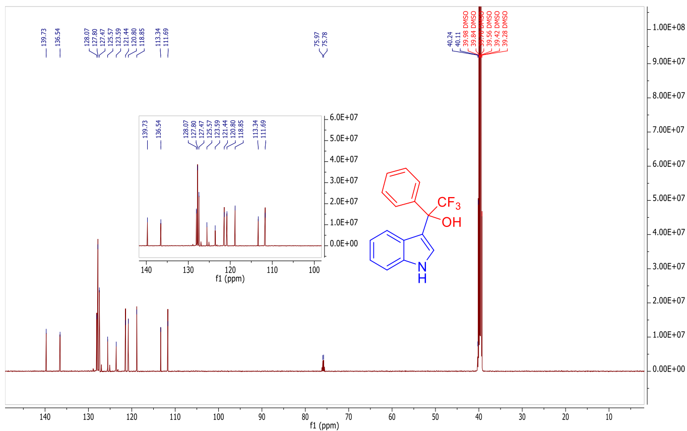
Figure S14. ^1\text{H} (600 MHz) and ^{13}\text{C} (151 MHz) Spectra of 2,2,2-trifluoro-1-(1 H -indol-3-yl)-1-phenylethan-1-ol ( 3p )
