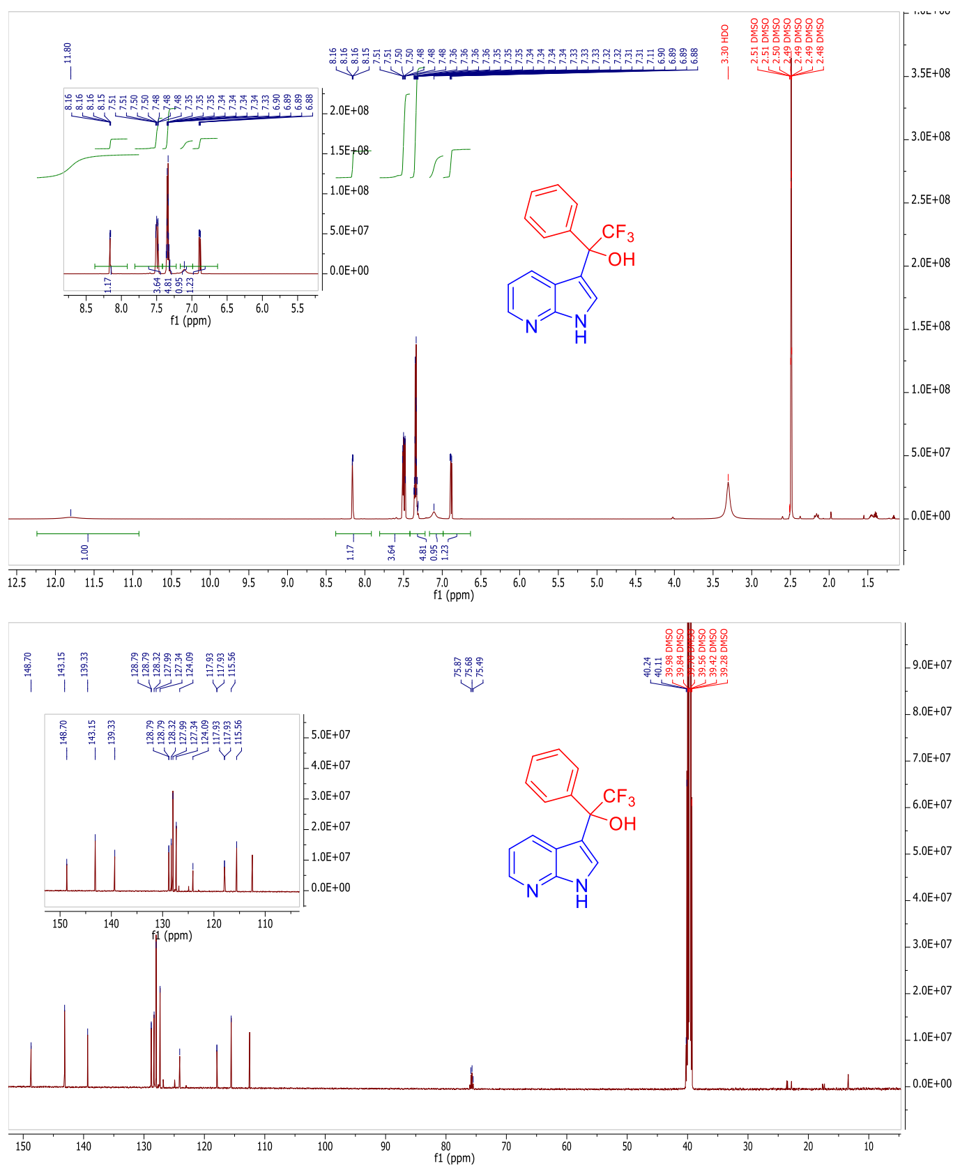
Figure S22. 1 H (600 MHz) and 13 C (151 MHz) Spectra of 2,2,2-trifluoro-1-phenyl-1-(1 H -pyrrolo[2,3- b ]pyridin-3-yl)ethan-1-ol ( 3x )
