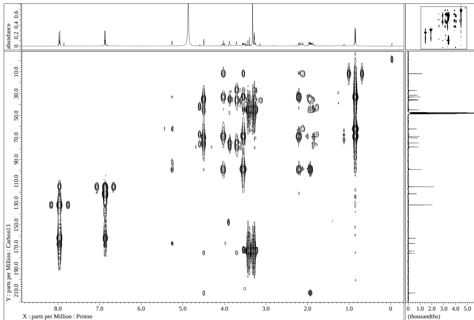
Figure S23 HMBC spectrum of 3 in CD 3 OD
