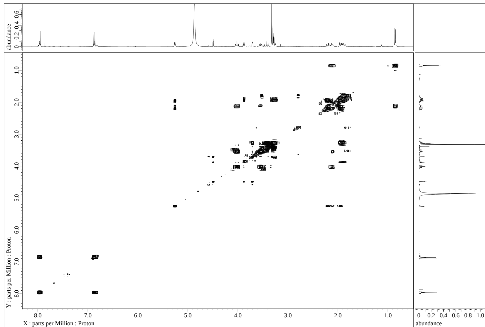
Figure S21 DQF-COSY spectrum of 3 in CD 3 OD
