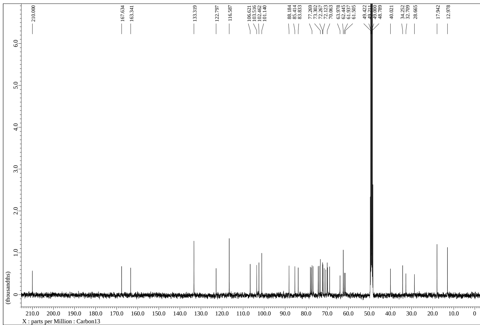
Figure S35 13 C NMR spectrum of 7 in CD 3 OD
