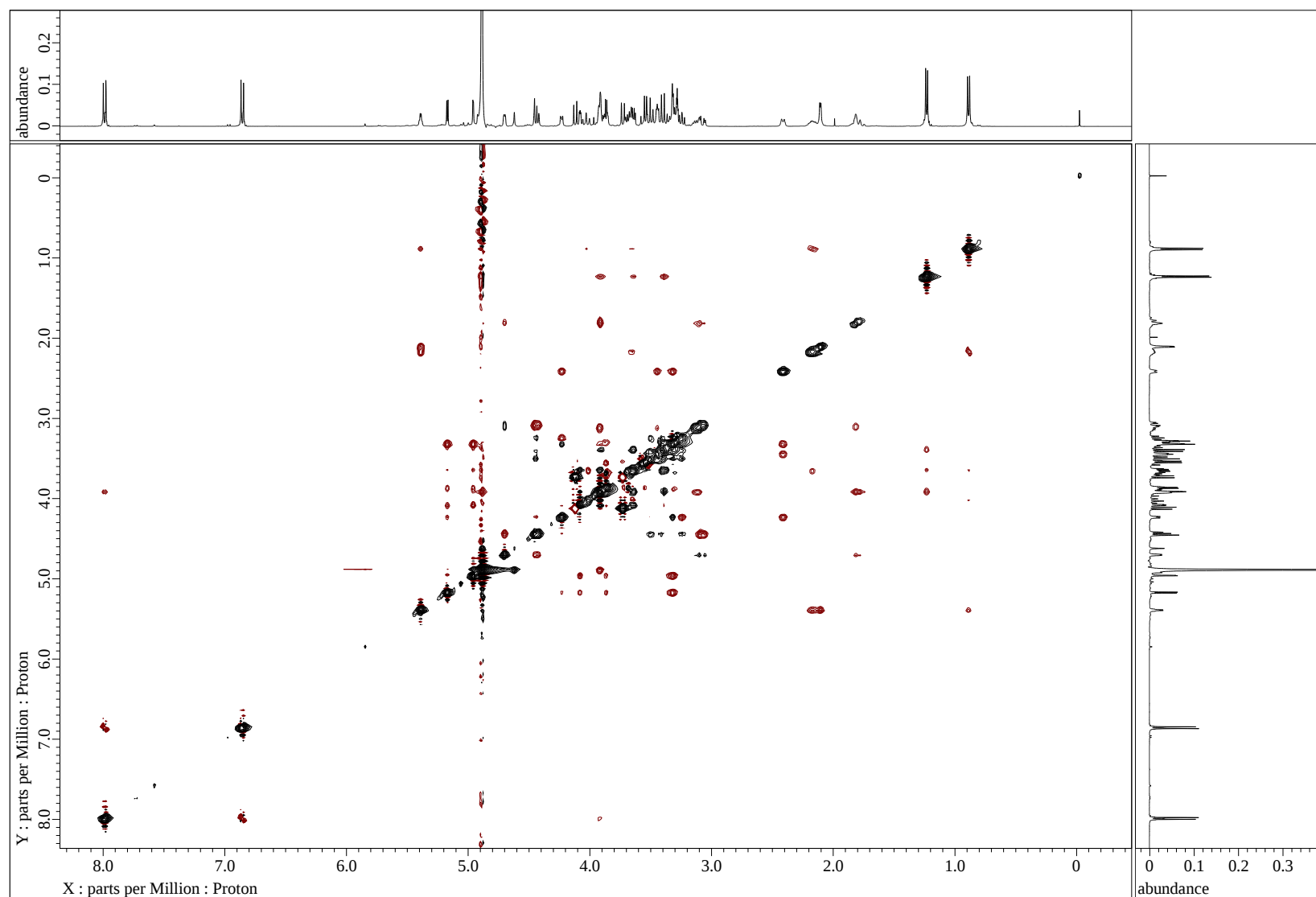
Figure S18 2D ROESY spectrum of 2 in CD 3 OD
