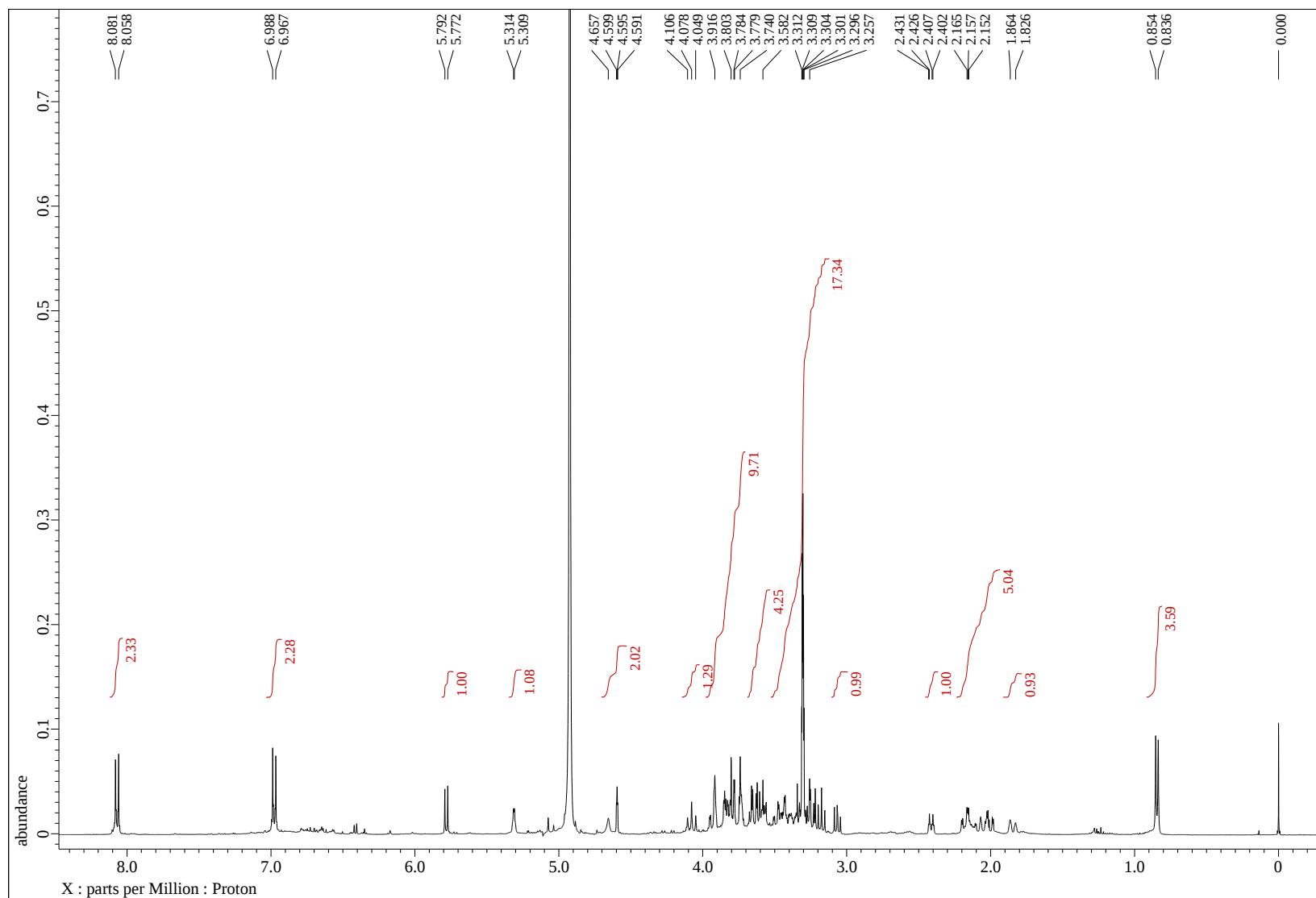
Figure S25 ^1\text{H} NMR spectrum of 4 in \text{CD}_3\text{OD}
