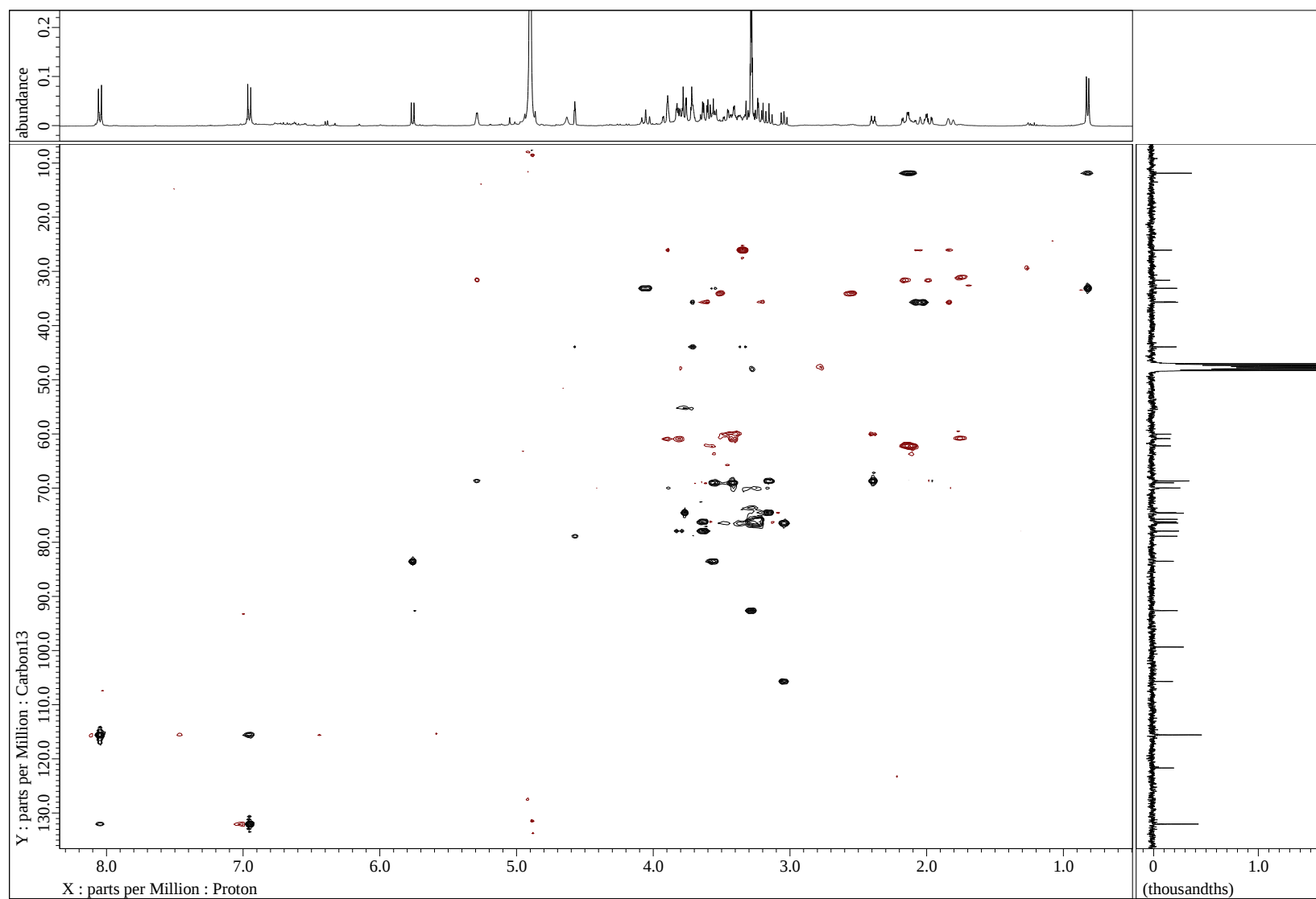
Figure S31 H2BC spectrum of 3 in CD 3 OD
