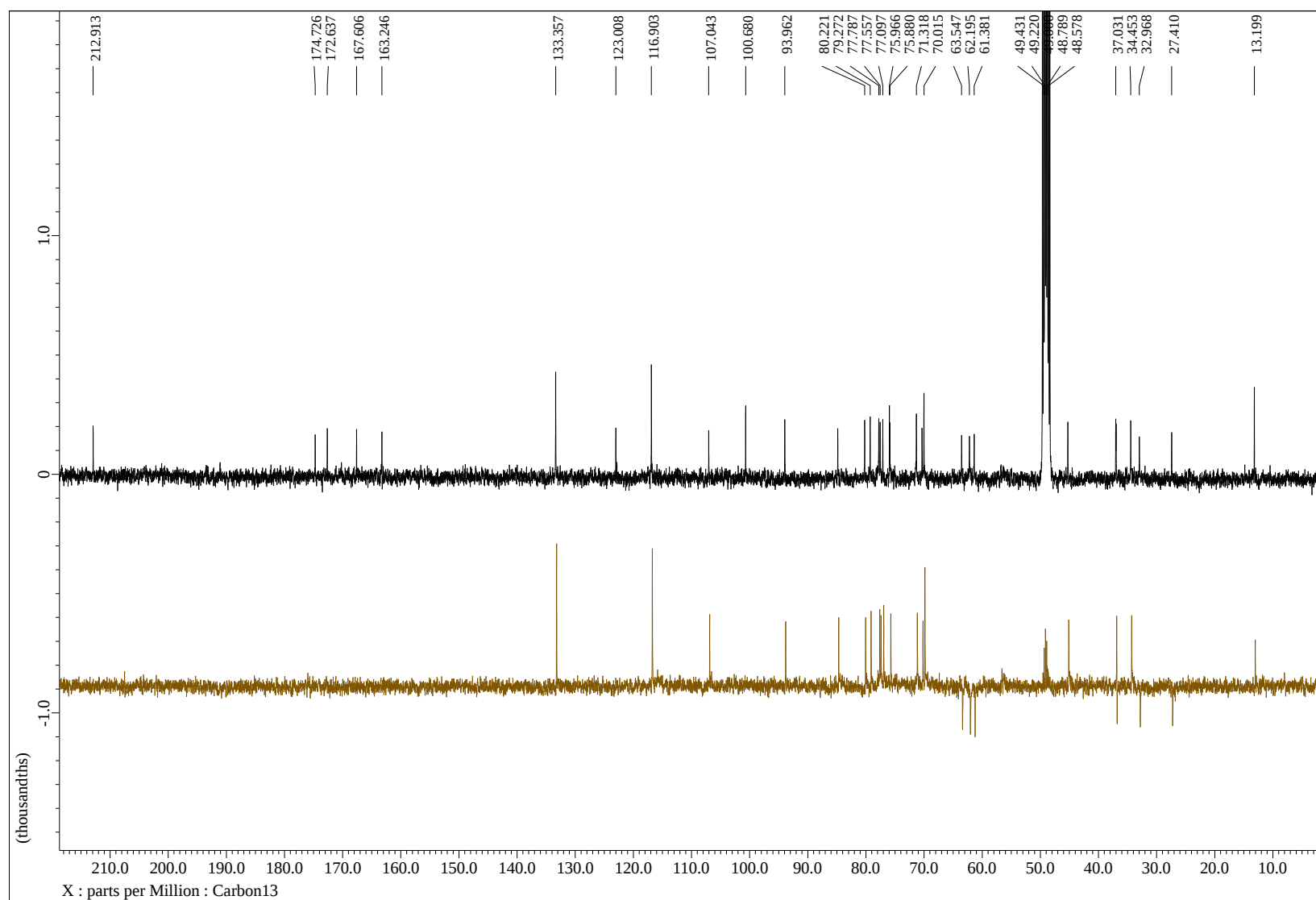
Figure S26 ^{13}\text{C} NMR and DEPT135 spectra of 4 in \text{CD}_3\text{OD}
