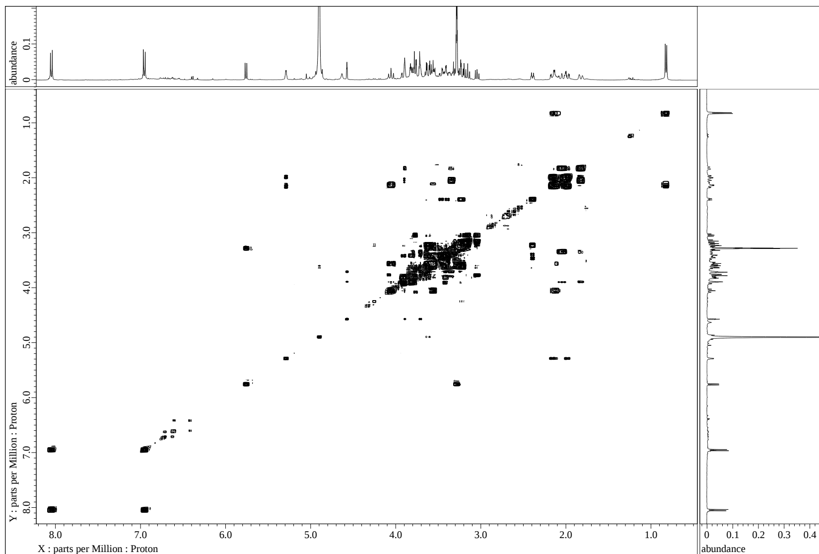
Figure S28 DQF-COSY spectrum of 4 in CD 3 OD
