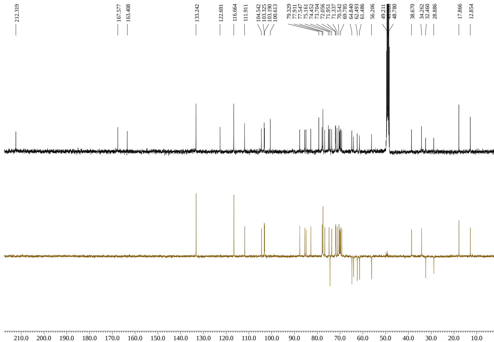
Figure S2 ^{13}\text{C} NMR and DEPT135 spectra of 1 in \text{CD}_3\text{OD}
