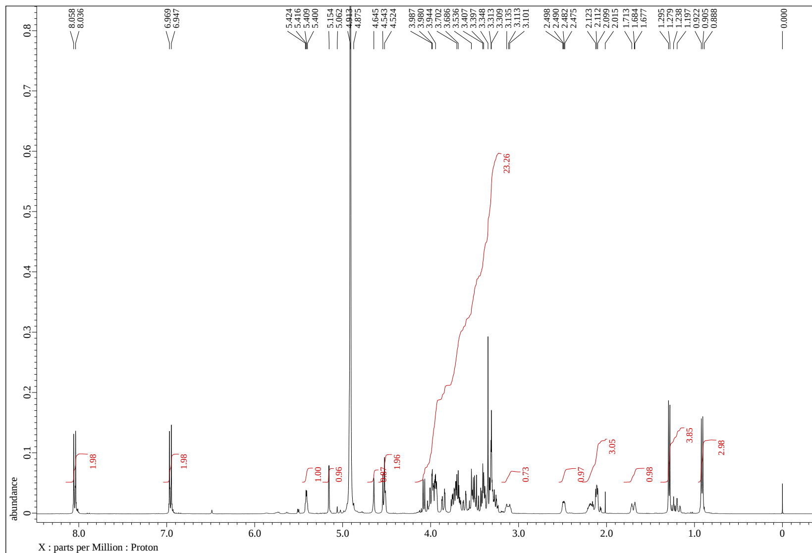
Figure S32 ^1\text{H} NMR spectrum of 6 in \text{CD}_3\text{OD}
