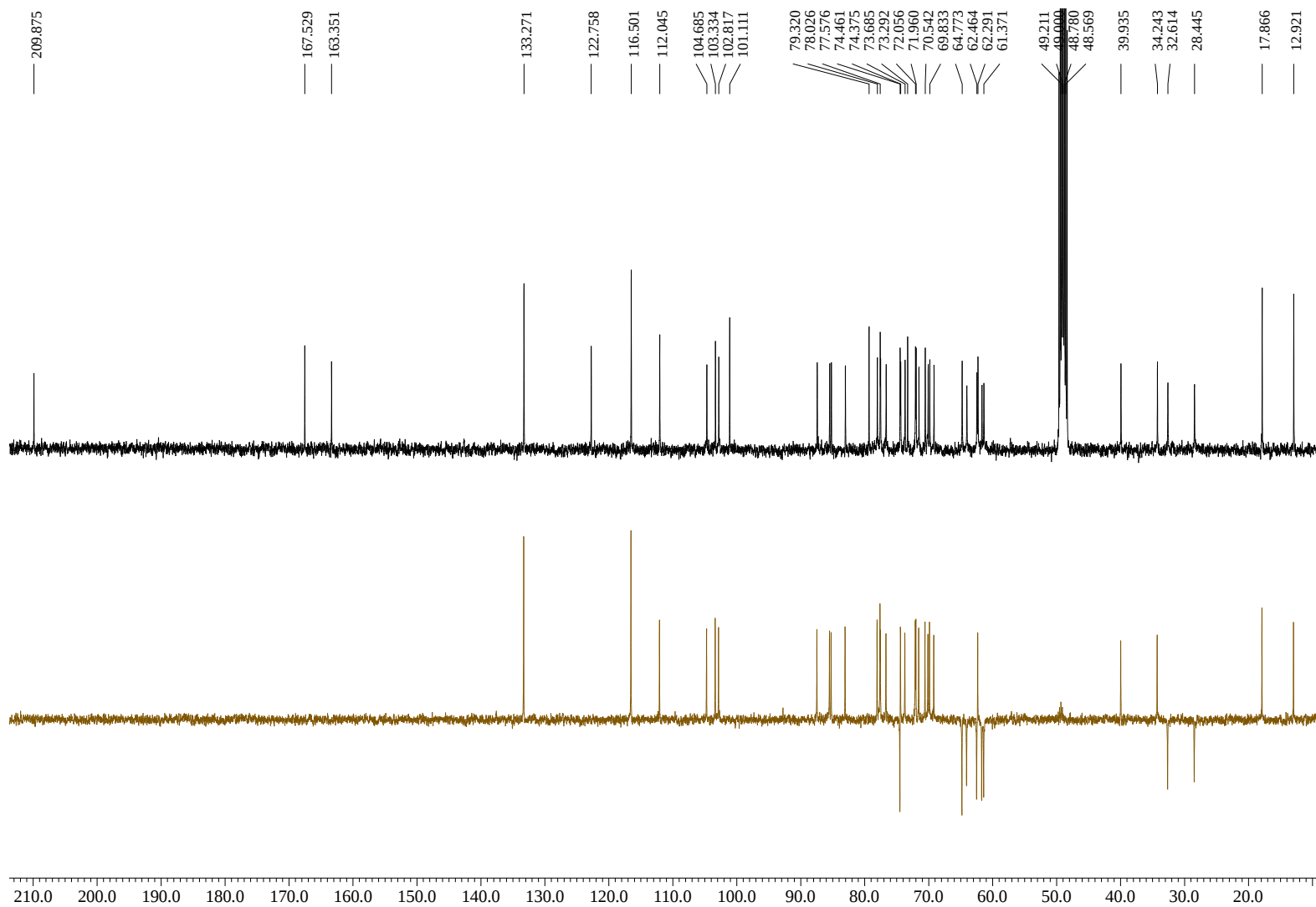
Figure S11 ^{13}\text{C} NMR and DEPT135 spectra of 2 in \text{CD}_3\text{OD}
