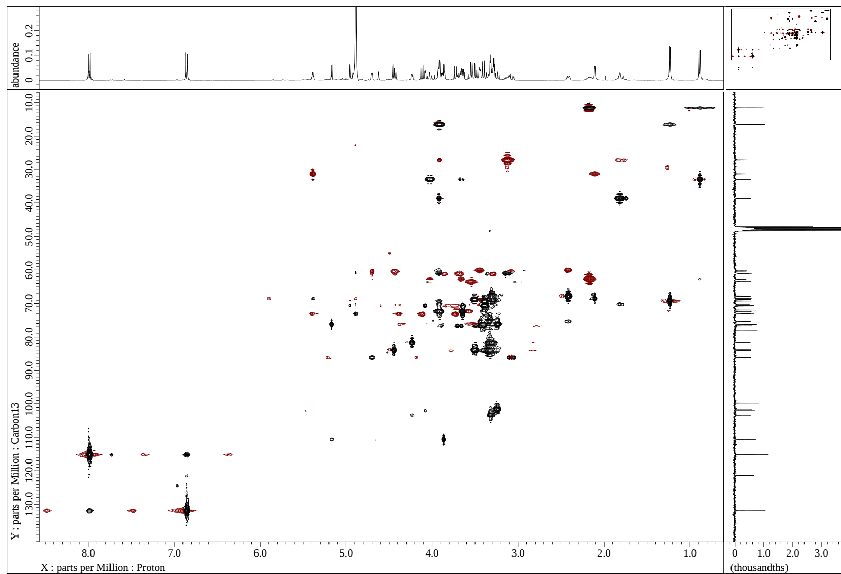
Figure S17 H2BC spectrum of 2 in CD 3 OD
