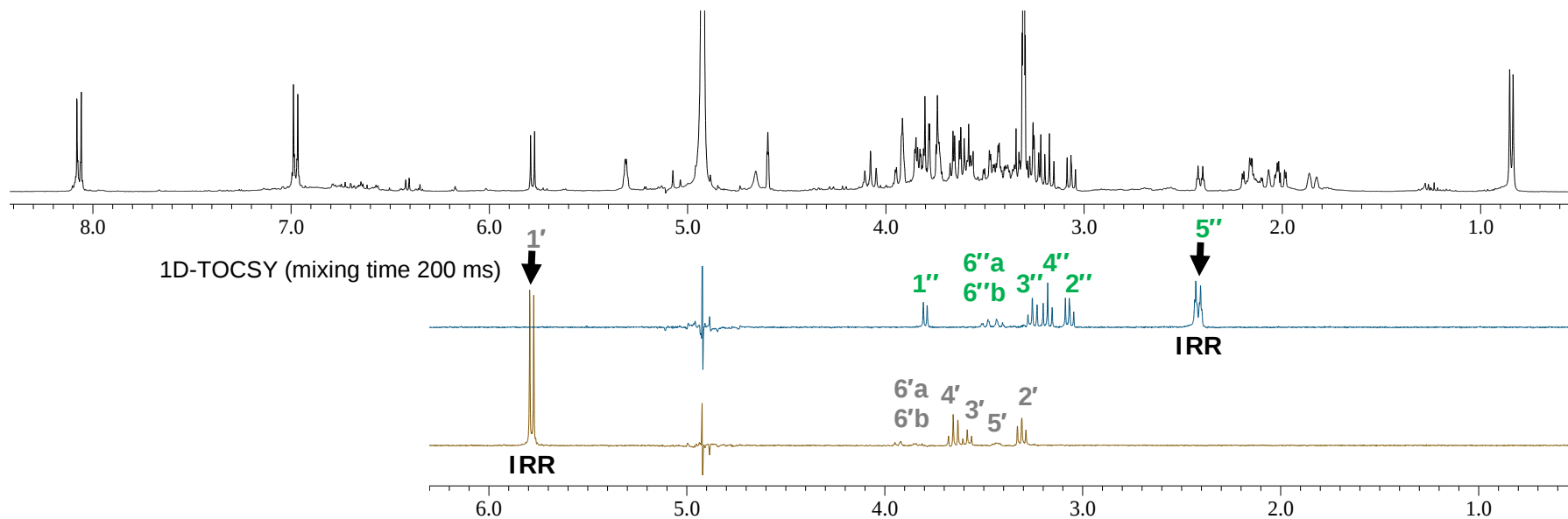
Figure S27 1D-TOCSY spectra of 4 in \text{CD}_3\text{OD}
