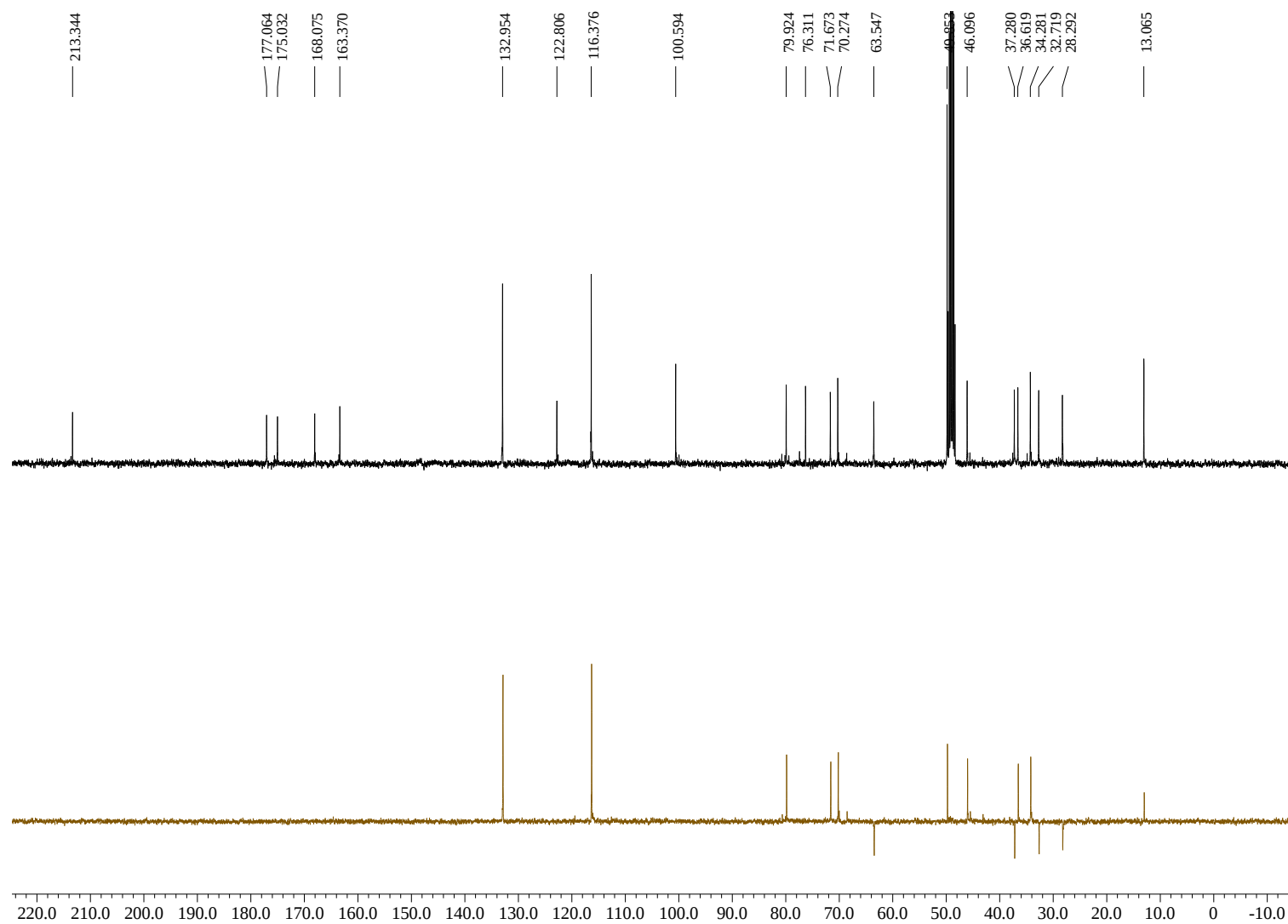
Figure S20 ^{13}\text{C} NMR and DEPT135 spectra of 3 in \text{CD}_3\text{OD}
