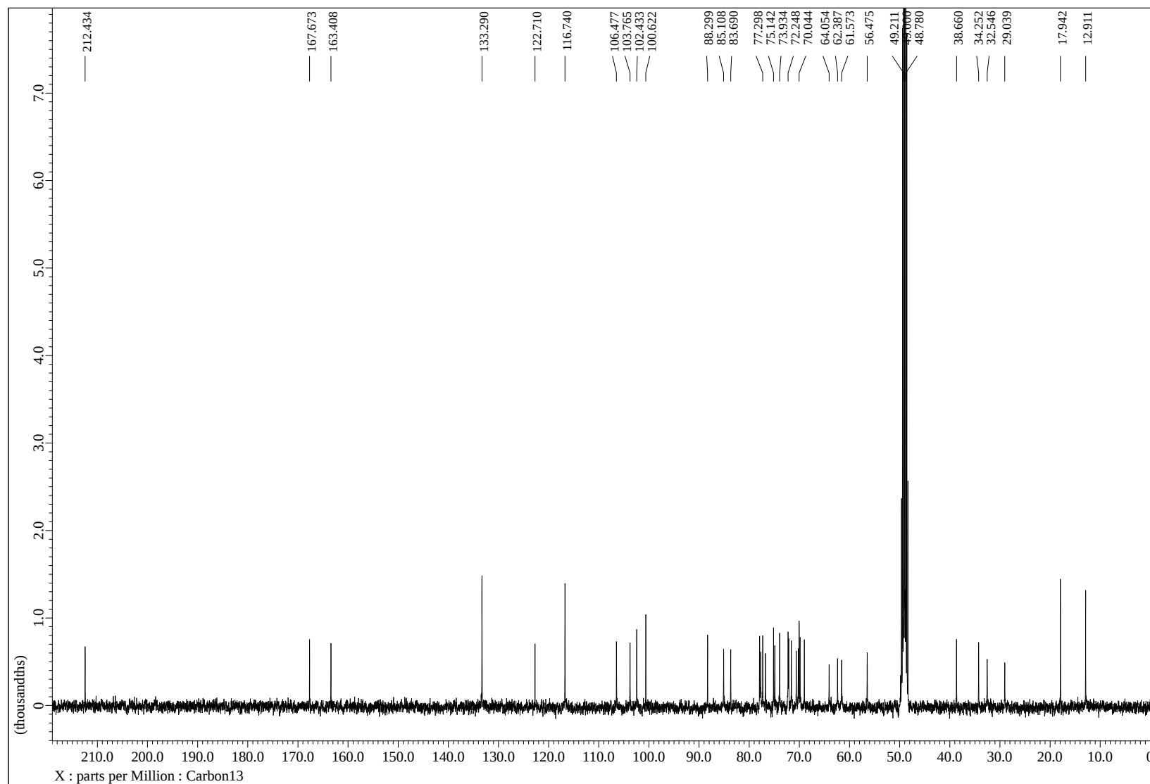
Figure S33 13 C NMR spectrum of 6 in CD 3 OD
