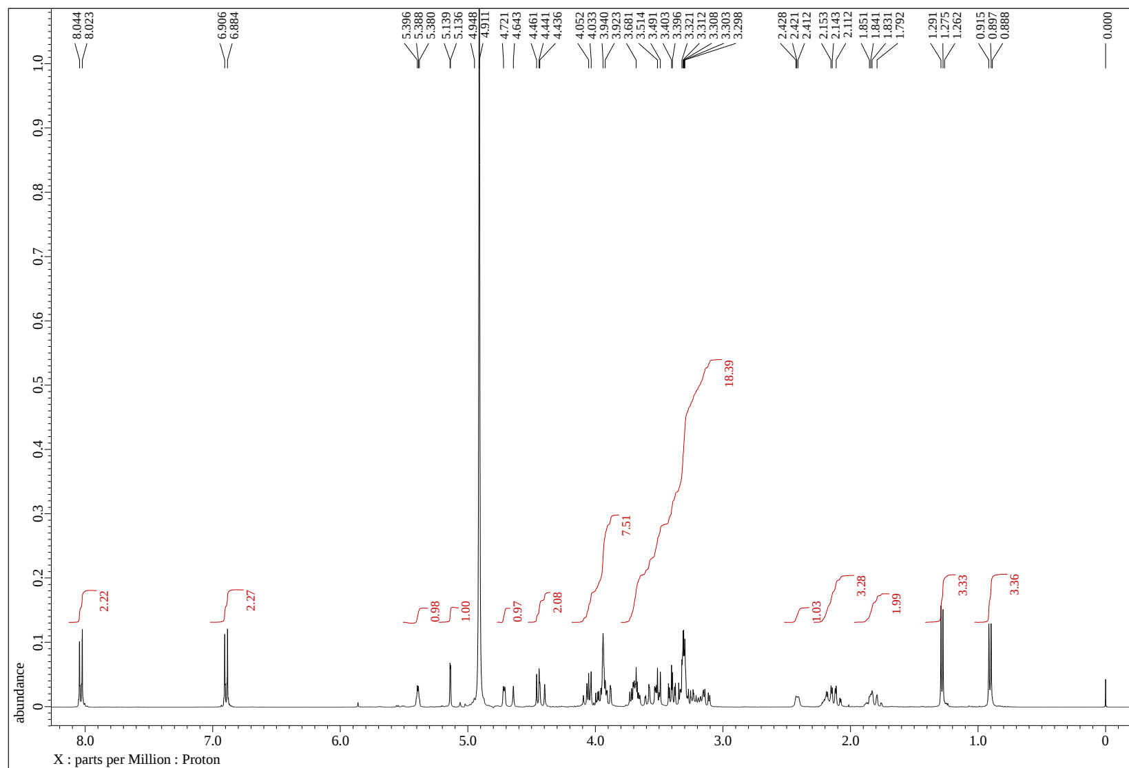
Figure S34 ^1\text{H} NMR spectrum of 7 in \text{CD}_3\text{OD}
