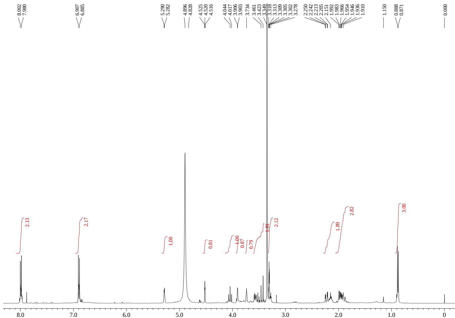
Figure S19 1 H NMR spectrum of 3 in CD 3 OD
