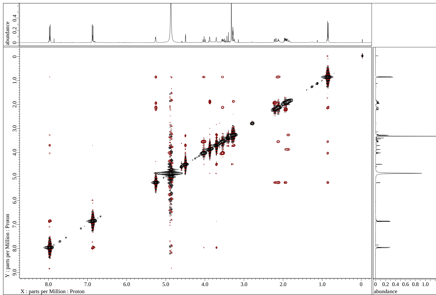
Figure S24 NOESY spectrum of 3 in CD 3 OD
