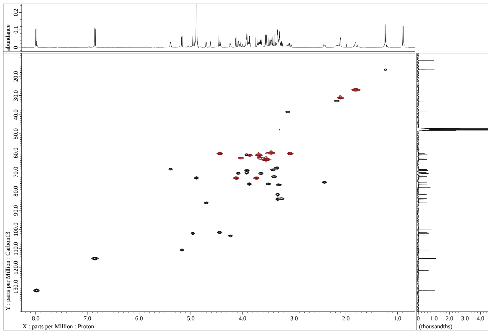
Figure S14 HSQC spectrum of 2 in CD 3 OD
