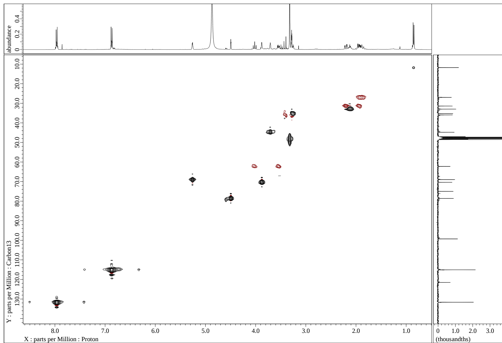
Figure S22 HSQC spectrum of 3 in CD 3 OD
