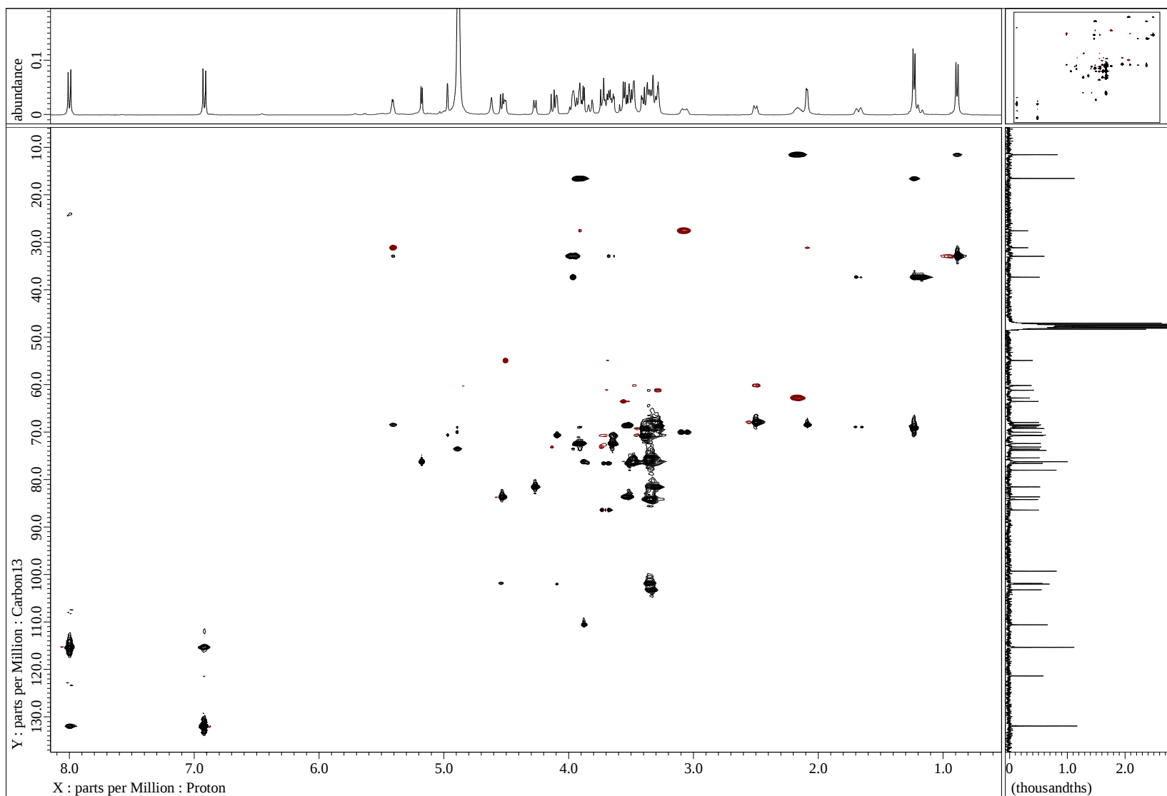
Figure S8 H2BC spectrum of 1 in CD 3 OD
