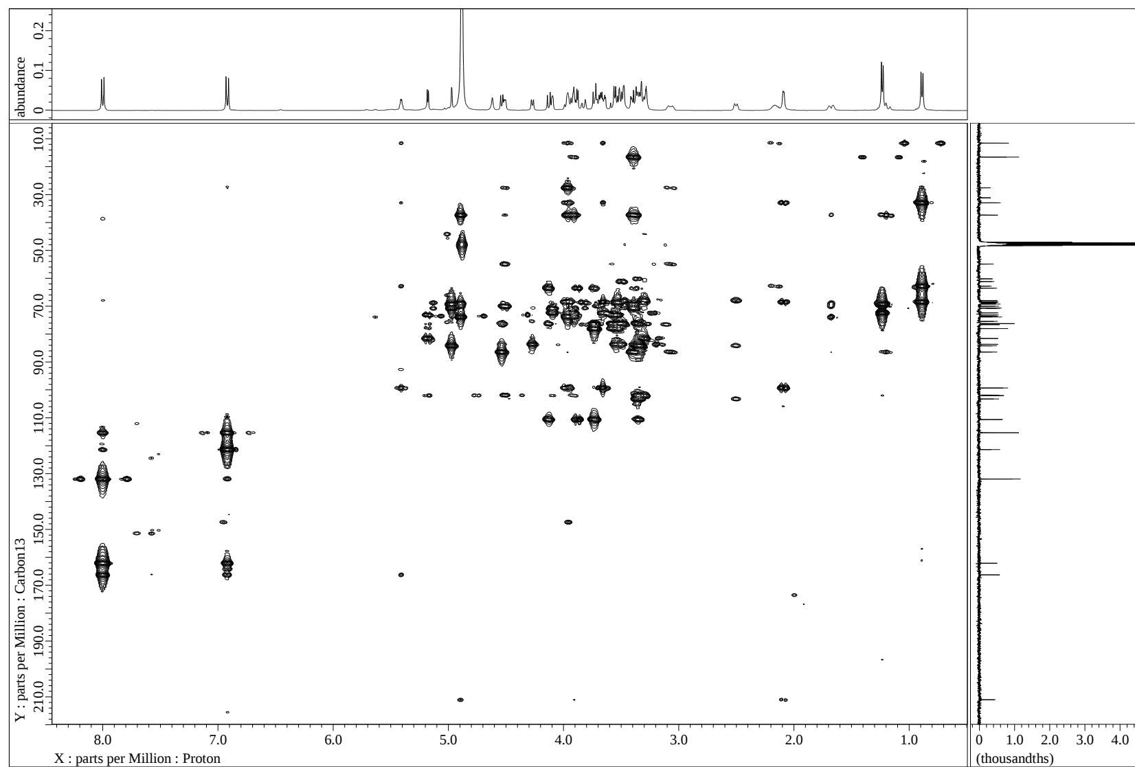
Figure S6 HMBC spectrum of 1 in CD 3 OD
