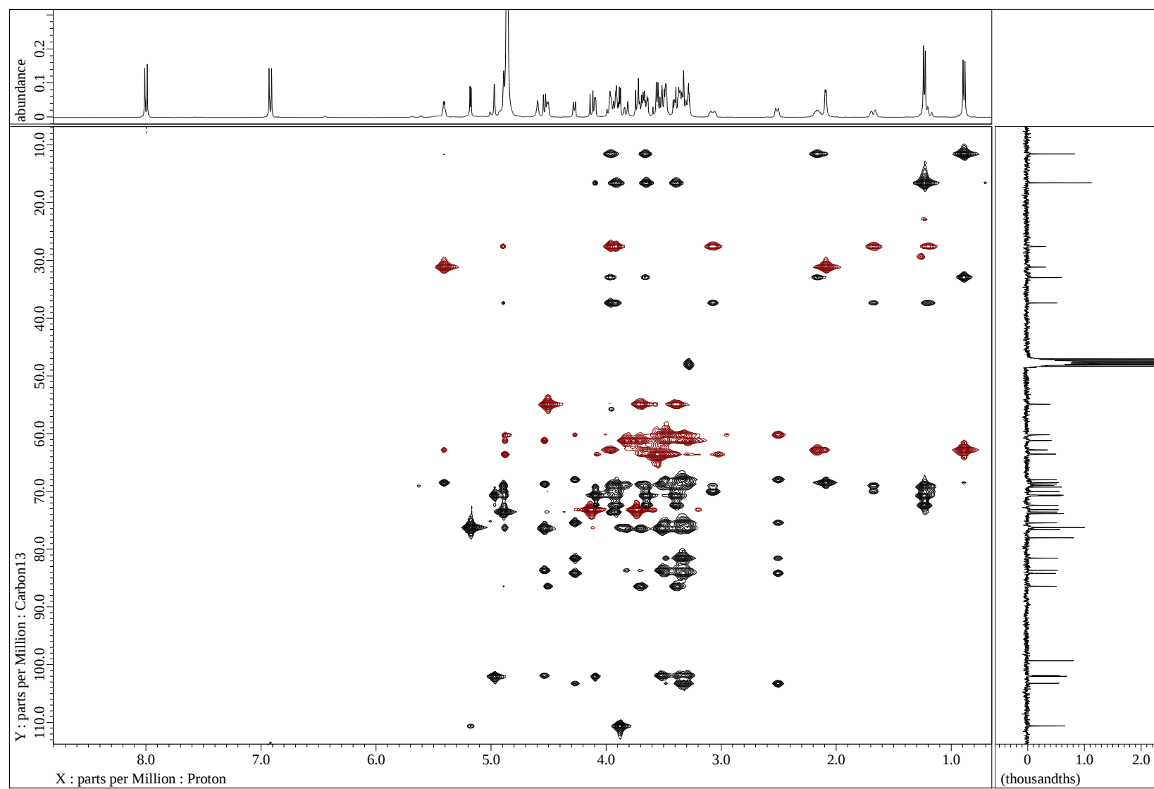
Figure S7 HSQC-TOCSY spectrum of 1 in CD 3 OD
