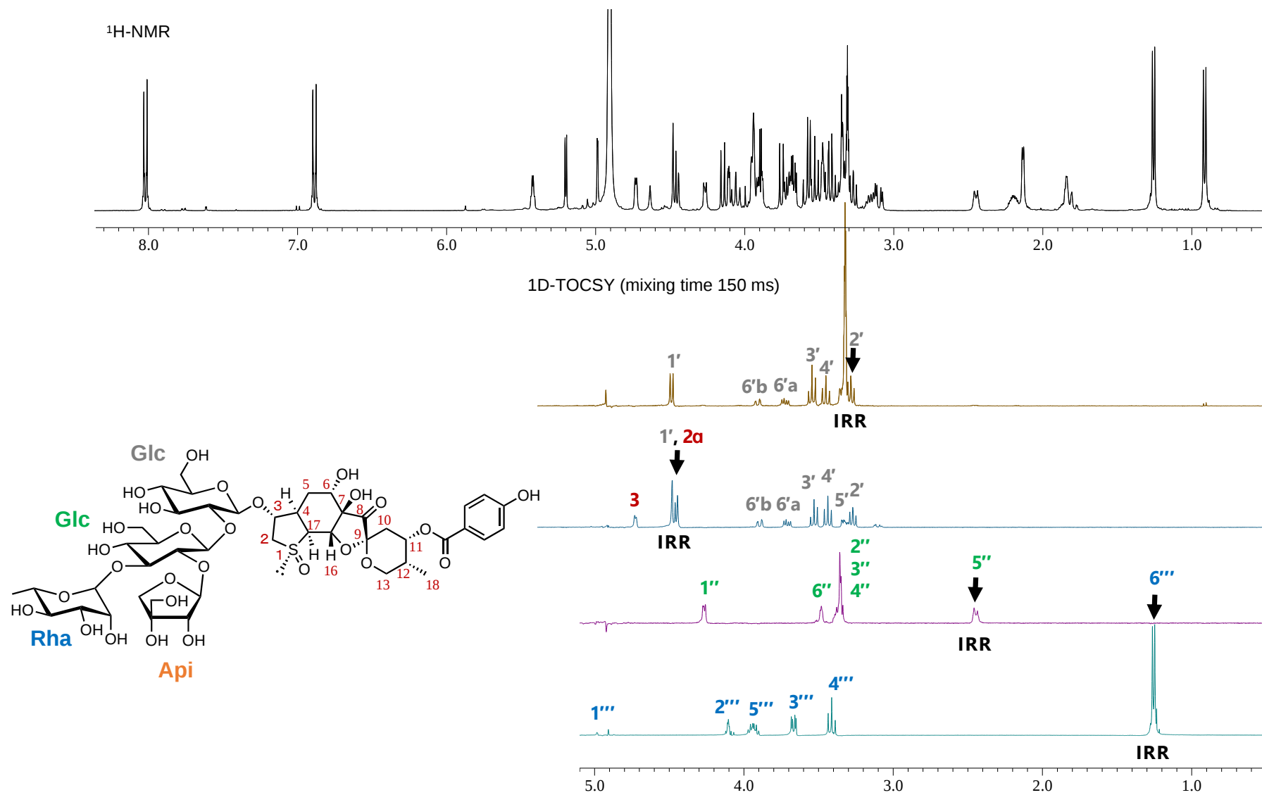
Figure S12 1D-TOCSY spectra of 2 in \text{CD}_3\text{OD}
