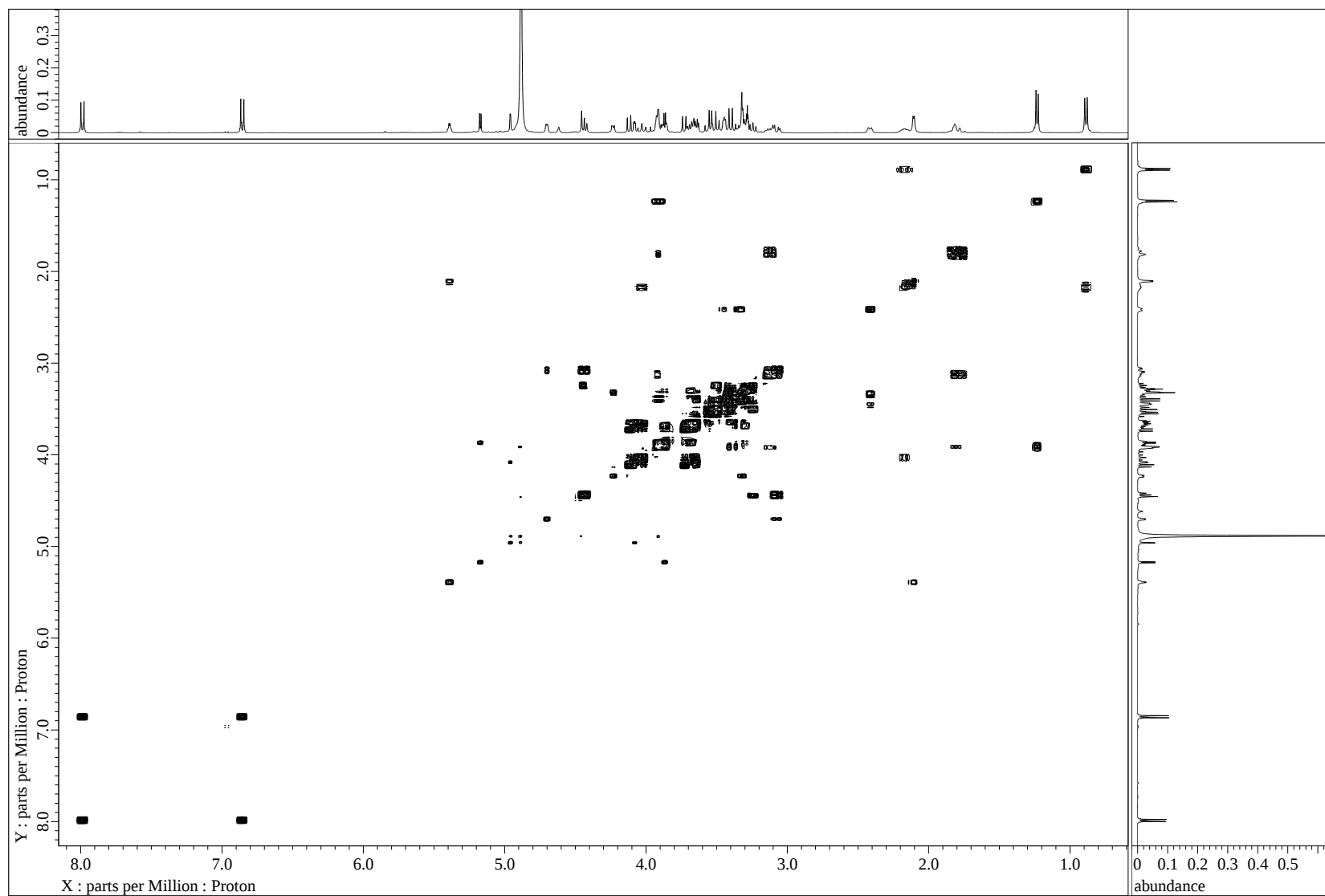
Figure S13 DQF-COSY spectrum of 2 in CD 3 OD
