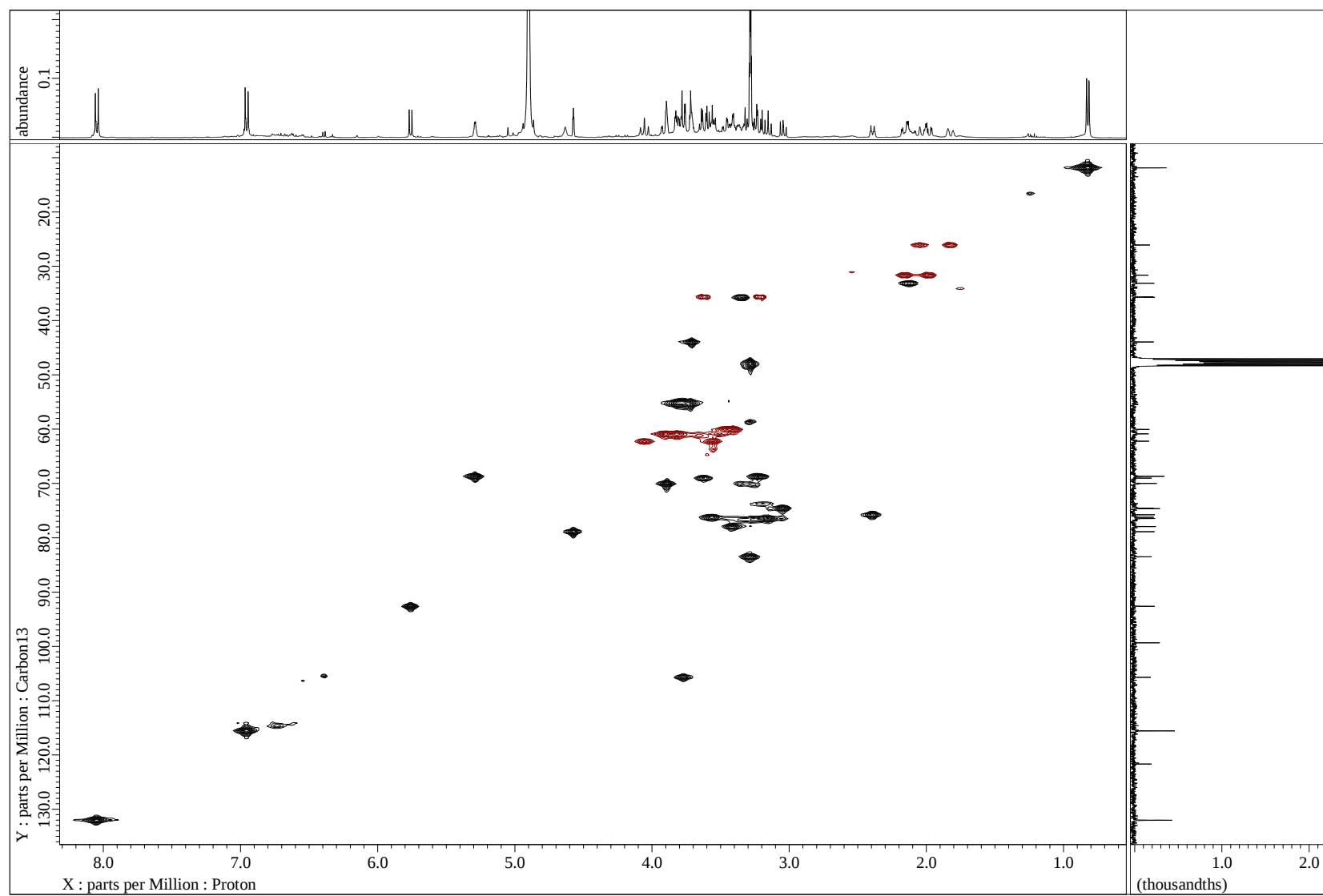
Figure S29 HSQC spectrum of 4 in CD 3 OD
