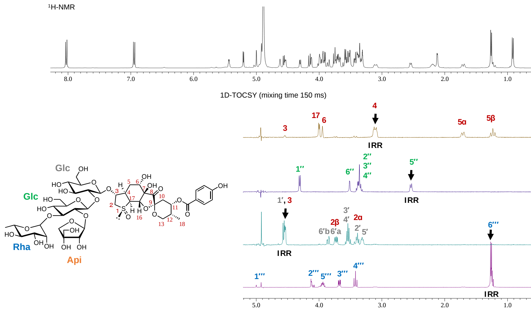
Figure S3 1D-TOCSY spectra of 1 in CD 3 OD
