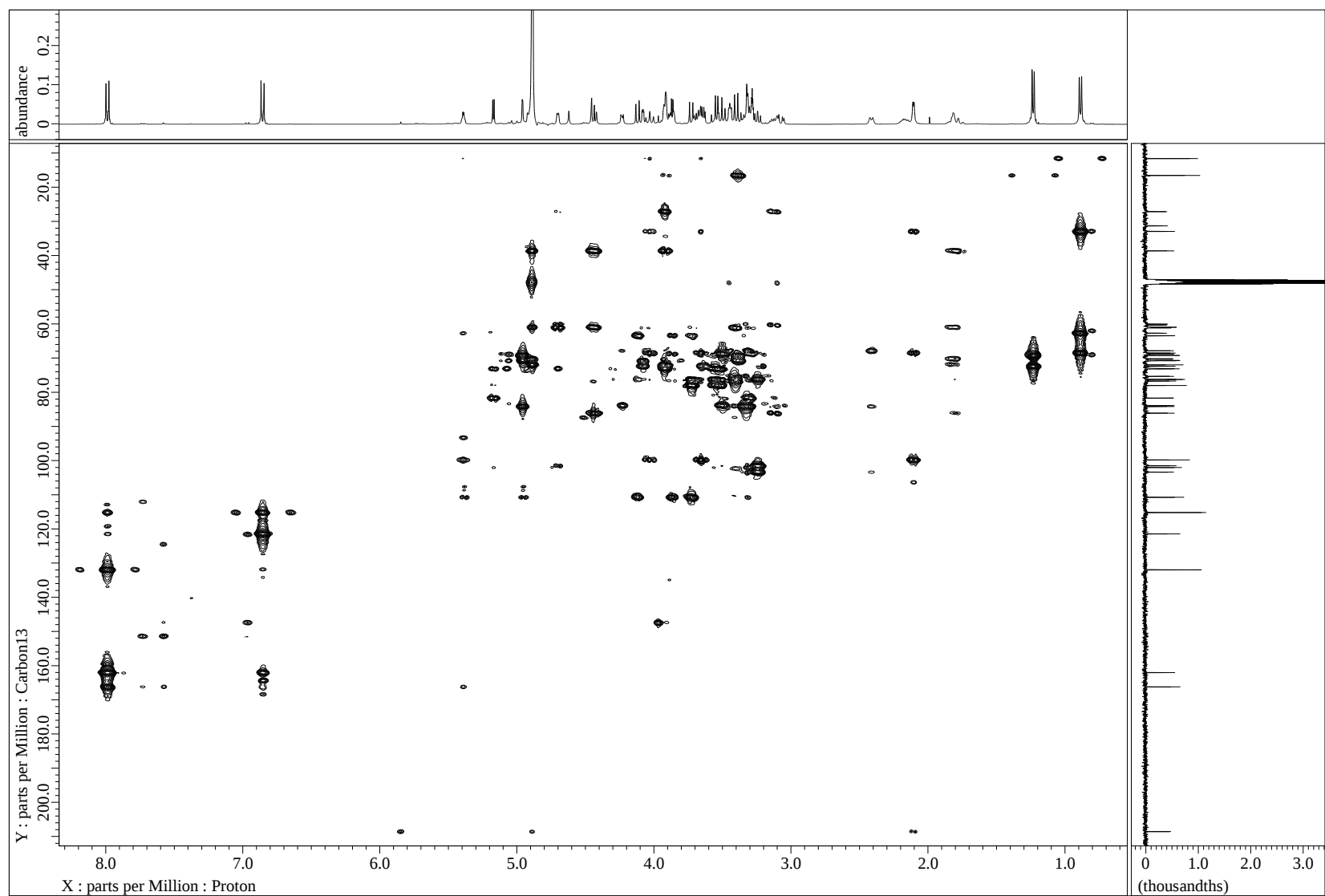
Figure S15 HMBC spectrum of 2 in CD 3 OD
