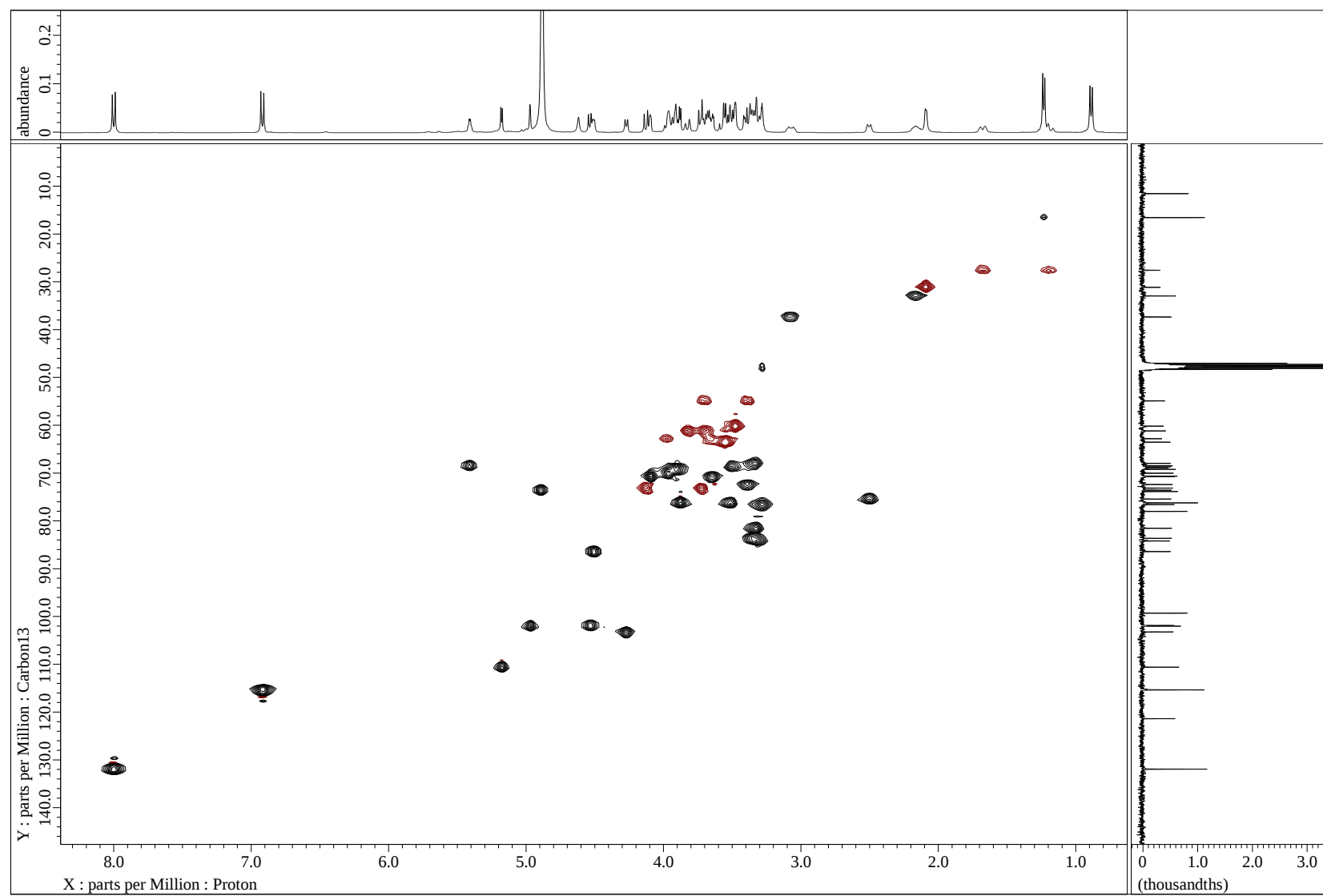
Figure S5 HSQC spectrum of 1 in CD 3 OD
