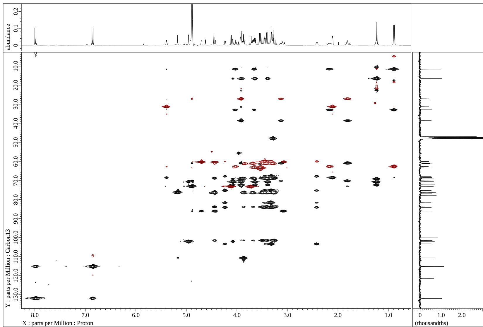
Figure S16 HSQC-TOCSY spectrum of 2 in CD 3 OD
