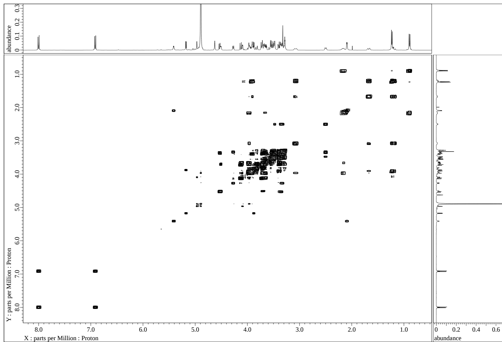
Figure S4 DQF-COSY spectrum of 1 in CD 3 OD
