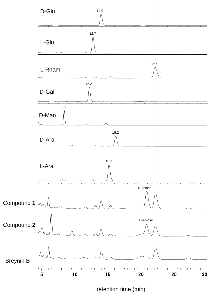
Figure S36 HPLC chromatograms for sugar identification
