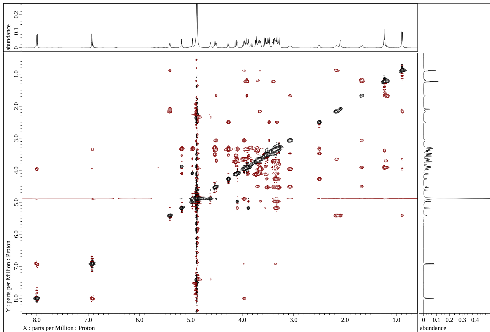
Figure S9 2D ROESY spectrum of 1 in CD 3 OD
