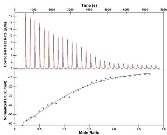
Figure S1: The ITC diagram of the TMeQ[6] to G.
