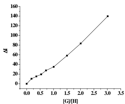
Figure S3: Stoichiometry plot for receptor 2 upon addition of \text{Cu}^{2+} ion from fluorescence.
