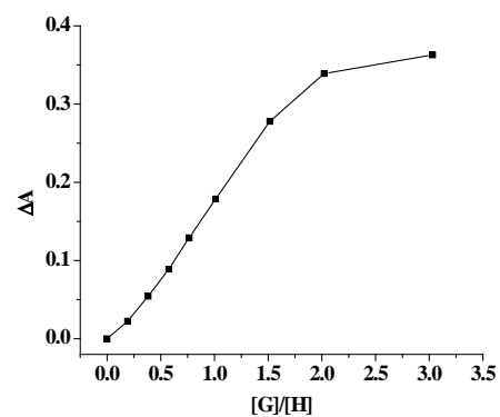
Figure S2: Stoichiometry plot for receptor 1 upon addition of \text{Cu}^{2+} ion from UV.
