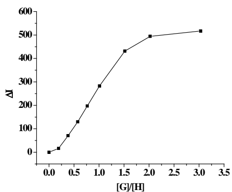
Figure S1: Stoichiometry plot for receptor 1 upon addition of \text{Cu}^{2+} ion from fluorescence.
