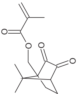
10-methacryloyloxycamphorquinone_1H.esp
