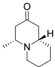
(-)-Epimyrtine
