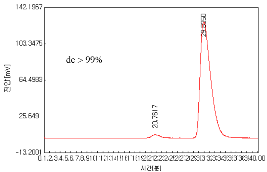
Figure S3: ^1\text{H} NMR and HPLC data of compound 7b .
