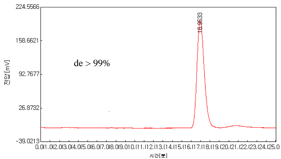
Figure S5: ^1\text{H} NMR and HPLC data of compound 7d .
