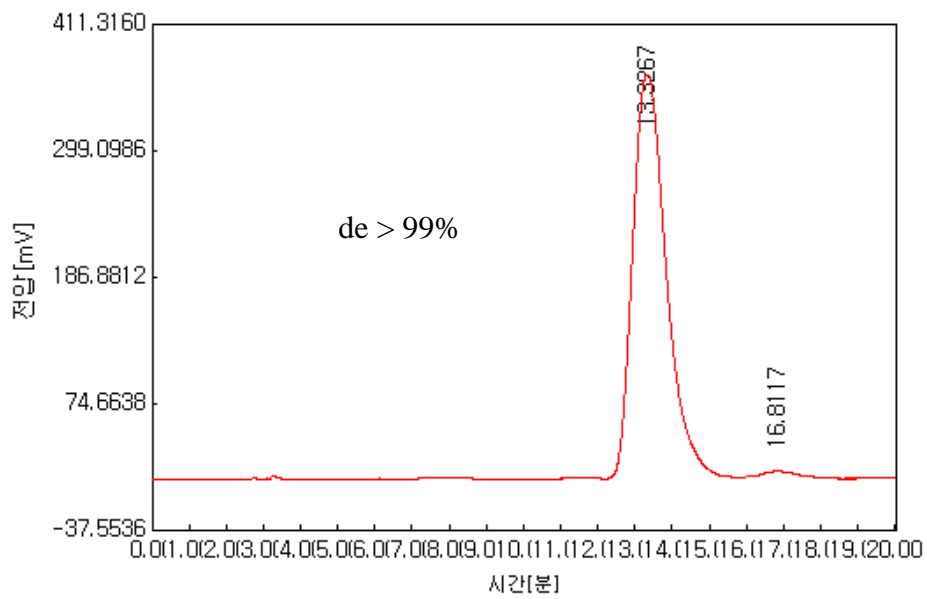
Figure S4: ^1\text{H} NMR and HPLC data of compound 7c .
