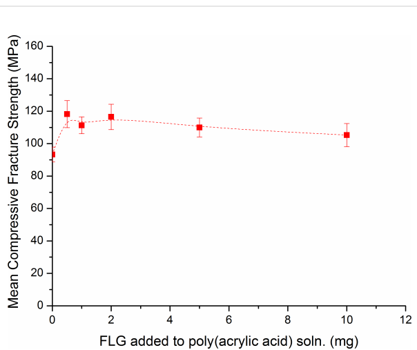
Figure 4: Change in mean compressive fracture strength with increasing graphene concentration.
