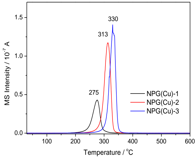
Figure S2: O 2 TPD spectra recorded on various fresh NPG(Cu) catalysts.
