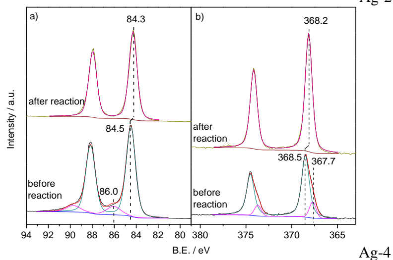
Figure S1: Au(4f) (a) and Ag (3d) (b) XP spectra recorded on various NPG(Ag) catalysts before and after reaction (1000 min on stream).
