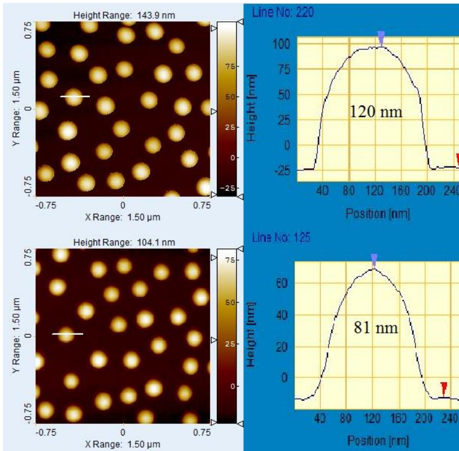
Figure S1: AFM measurements of the height from the gold film surface to the gold cap on the top the PS particle (To the right a single line scan is shown). Upper picture: No heating. Lower picture: Heated to 125 °C.
