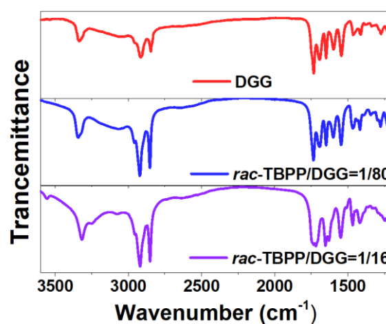
Figure S7. FTIR absorption spectra of rac -TBPP/DGG gels at molar ratios of 1:80 and 1:16.
